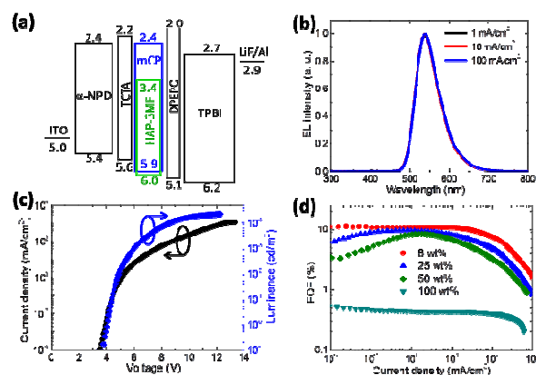
Fig. 4 EL characteristics of an ExOLED containing an 8 wt% HAP-3MF:mCP blend film as an emitting layer. (a) Device structure and energy level diagram (values are in eV). (b) EL spectra recorded at various current densities. (c) Current density-voltage-luminance ( J-V-L ) characteristics. (d) EQE as a function of current density.
