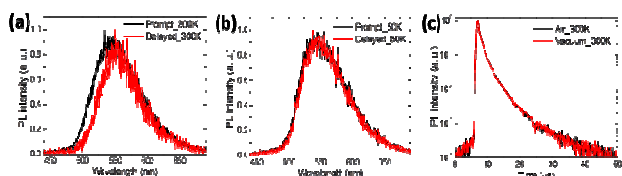
Fig. 3 Transient PL decay properties of an 8 wt% HAP-3MF:mCP exciplex system. (a) Prompt and delayed PL spectra under vacuum condition at 300 K. (b) Prompt and delayed PL spectra under vacuum condition at 50 K. (c) Transient PL decay in air and under vacuum conditions at 300 K.
