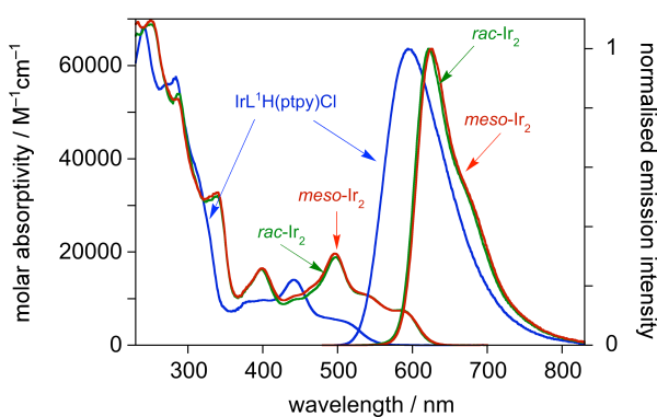
Figure 1 Absorption and photoluminescence spectra of \text{IrL}^{\text{I}}\text{H}(\text{ptpy})\text{Cl} (blue lines) and the rac and meso forms of \text{Ir}_2\text{L}^{\text{I}}(\text{ptpy})_2\text{Cl}_2 (green and red lines respectively) in solution in \text{CH}_2\text{Cl}_2 at 298 K.
