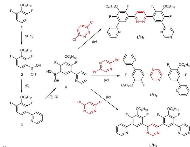
Scheme 1. Synthesis of cyclometallating bis-terdentate ligands. (i) BuLi; (ii) B(O i Pr) 2 ; then H 3 O + ; (iii) 2-bromopyridine, Pd cat.; (iv) Pd cat.
