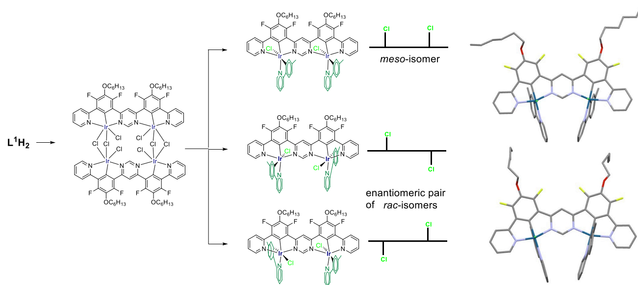
Scheme 2. Synthesis of \text{Ir}_2\text{L}^1(\text{pty})_2\text{Cl}_2 ; schematic illustration of the relative disposition of the Cl ligands (centre), and corresponding structures obtained by X-ray diffraction (right; for clarity, the structures are shown without H atoms, solvent molecules and minor disorder components).
