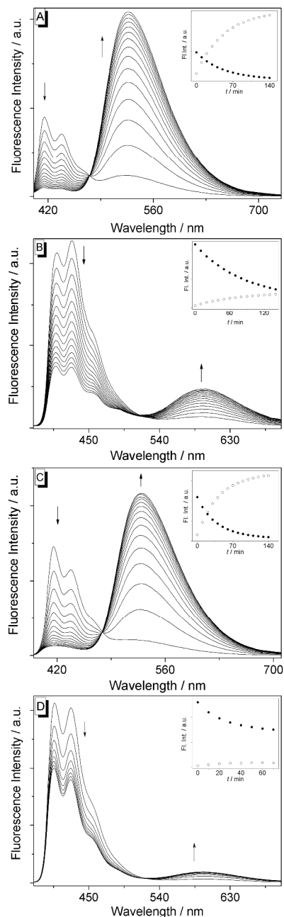
Fig. 1. Fluorimetric monitoring of the reaction of H_2O_2 (1.0 mM) with 1a (A, 10 \mu M , \lambda_{ex} = 366 nm), 1b (B, 10 \mu M , \lambda_{ex} = 361 nm), 1c (C, 10 \mu M , \lambda_{ex} = 366 nm), or 1d (D, 10 \mu M , \lambda_{ex} = 366 nm) in phosphate buffer (0.1 M, pH = 7.4). Arrows indicate the development of emission bands with time. Inset: Plot of the fluorescence maxima of 1a-d (●) and 2a,b (○) versus time.
