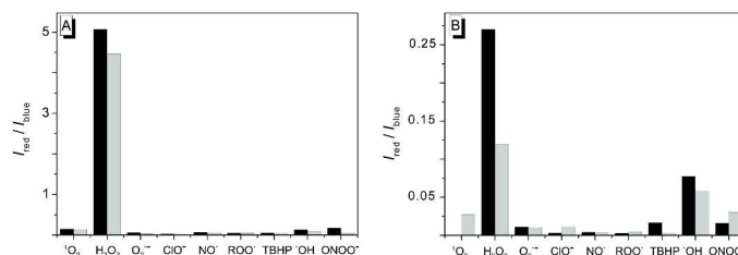
Fig. 2. Ratiometric fluorimetric analysis of the reaction of 1a (A, black), 1c (A, grey), 1b (B, black), and 1d (B, grey) ( c = 10 \mu M ) with selected ROS ( c = 1.6 \times 10^{-4} M , resp.) in phosphate buffer ( c = 0.1 M , pH = 7.4); t = 60 min; 1a , 1c : \lambda_{ex} = 366 nm, 1b , 1d : \lambda_{ex} = 361 nm; ROO^{\cdot-} = C_4H_9N_2OO^{\cdot-} .
