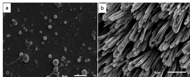
Figure 1: Morphological characterization by scanning electron microscopy of the structures assembled by WW-((CT) 5 T 2 ): a) spherical structures assembled at low concentration (below 1 mM) whereas b) fibres develop under controlled aggregation (time and temperature).
