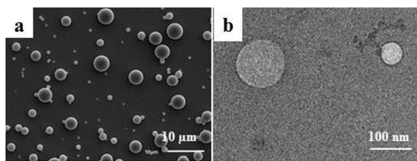
Figure 2: Spherical structures of WW dipeptide in aqueous solution of HFIP as observed by a) scanning electron microscopy and b) transmission electron microscopy.
