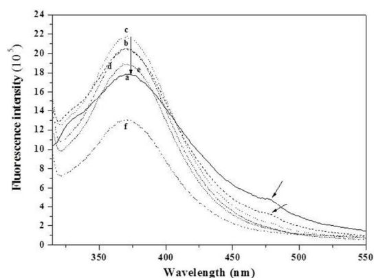
Figure 4: Fluorescence emission spectra for decreasing concentrations of the WW-DNA hybrid. (a) 2 mM, (b) 1 mM, (c) 0.5 mM, (d) 0.25 mM, (e) 0.13 mM and, (f) 0.06 mM
