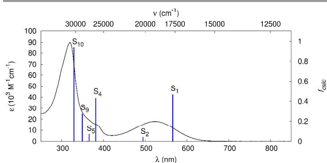
Fig. 2 Electronic absorption spectrum of 1 in THF solution, together with the calculated S 0 →S n transitions using the PBE0 xc-functionals.
