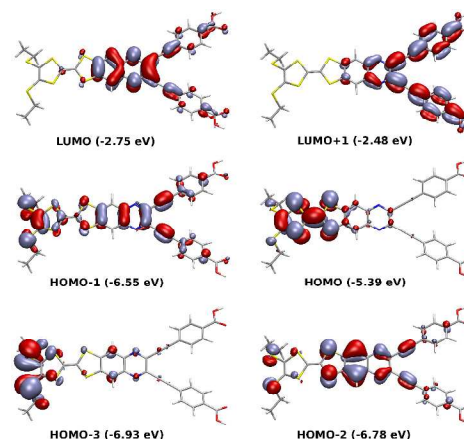
Fig. 3 Molecular orbitals of 1 that are involved in the main transitions.
