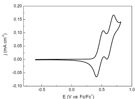
Fig. 1 Cyclic voltammogram of 1 in THF (0.1 M Bu 4 NPF 6 ; Pt working electrode; scan rate 50 mVs -1 ).
