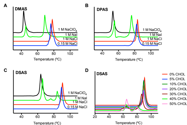
Fig. 2. Differential scanning calorimetry of AS lipids in the presence of additives. Transition temperature reduction using the Hofmeister series of chaotropic salts ( \text{NaClO}_4 > \text{NaI} > \text{NaCl} ) on (A) DMAS, (B) DPAS, (C) DSAS. Effect of cholesterol on the transition temperature of DSAS.
