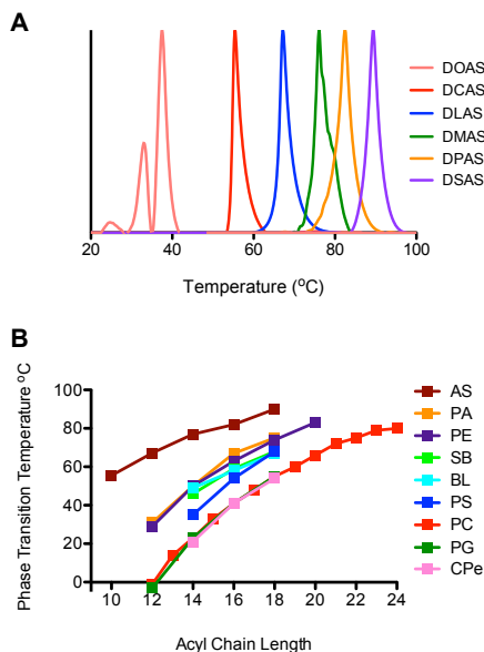
Fig. 1. Differential scanning calorimetry of AS lipids. (A) T_m comparison of all AS lipids in 150 mM NaCl salt. (B) Phase transition temperatures of AS lipids in comparison to other commercially available and inverse charge lipids. PC, phosphatidylcholine; CPe, ethylated inverse PC lipid; PG, phosphatidylglycerol; PS, phosphatidyl serine; BL, betaine-like; SB, inverse sulfobetaine; PE, phosphatidylethanolamine; PA, phosphatidic acid; AS, inverse sulfolipids.
