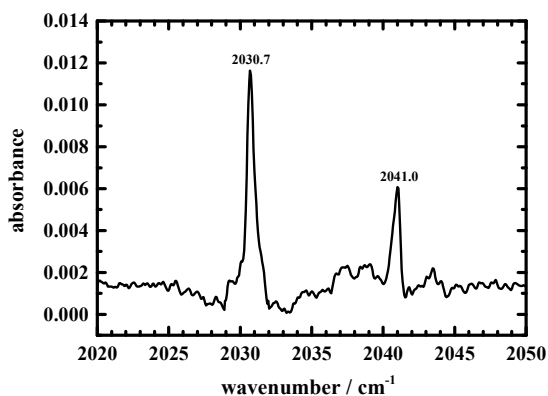
Figure 2. Absorption spectrum after irradiation of ^{12}\text{C}^2\text{H}_4 : ^1\text{H}_2 :Ne =
