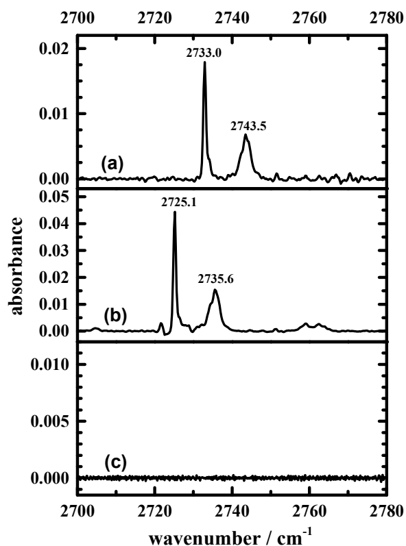
Figure 1. Absorption spectra after irradiation of methane: \text{H}_2:\text{Ne} = 1:6:1000 at 121.6 nm: (a) ^{12}\text{C}^1\text{H}_4: ^1\text{H}_2:\text{Ne} for 450 min, (b) ^{13}\text{C}^1\text{H}_4: ^1\text{H}_2:\text{Ne} for 510 min, (c) ^{12}\text{C}^2\text{H}_4: ^1\text{H}_2:\text{Ne} for 510 min, all at 3 K; resolution 0.5\text{ cm}^{-1} , from 600 coadded interferograms.
