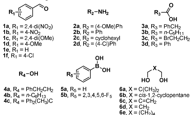
Fig. 1. Compounds examined in this study.
