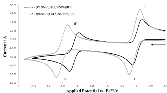
Figure 1. Cyclic voltammetry of 2a and 2b (1.5 mM solution in THF, 0.1M [\text{Bu}_4\text{N}][\text{PF}_6] ) recorded at 100 \text{mV s}^{-1} .
