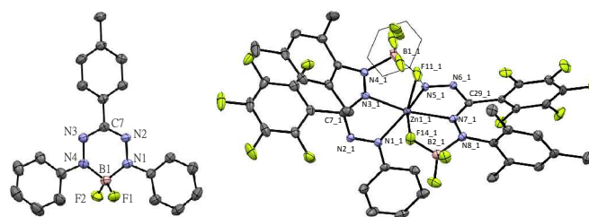
Figure 2. Molecular structure of 3a (left) and 4b (right) showing 50% probability ellipsoids. For 3a , [\text{Cp}_2\text{Co}]^+ cation and THF molecule are omitted; for 4b , one of the two independent molecules is shown; for both, hydrogen atoms are omitted for clarity.
