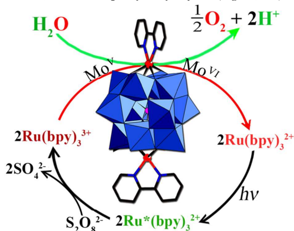
Scheme 1. Compound 1 catalyzes water oxidation to generate \text{O}_2 under the visible light irradiation, using [\text{Ru}(\text{bpy})_3]^{2+} as photosensitizer and \text{S}_2\text{O}_8^{2-} as sacrificial electron acceptor.
