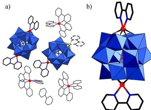
Fig. 1 a) The asymmetric unit of 1 contains one (\text{Co}^{\text{II}}\text{bpy})_2(\text{PMo}_8^{\text{VI}}\text{Mo}_4^{\text{VO}}\text{O}_{40})^{3-} unit and one [(\text{Co}^{\text{II}}\text{bpy})_{1.5}(\text{PMo}_8^{\text{VI}}\text{Mo}_4^{\text{VO}}\text{O}_{40})]^{4-} unit along with three \text{Co}^{\text{II}}(\text{bpy})_3 and one \text{H}_2\text{bpy} cations. b) The bicapped Keggin structure showing coordination of the \text{Co}^{\text{II}}\text{bpy} unit to four terminal oxygen atoms of the POM. All of the hydrogen atoms and lattice water molecules have been omitted for clarity. Colour code: blue polyhedra: Mo; red ball: Co; yellow ball: disordered Co; violet: P; black: C; blue: N. The disordered \text{Co}^{\text{II}}(\text{bpy}) subunit is shown with dotted lines.
