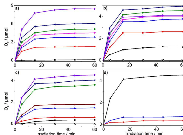
Fig. 2 Photochemical \text{O}_2 production from borate buffer solution (80 mM, pH = 9.0). a) 1.0 mM [\text{Ru}(\text{bpy})_3]\text{Cl}_2 , 5.0 mM \text{Na}_2\text{S}_2\text{O}_8 , and various concentrations of 1 (from bottom to top): 0, 2.5, 3.75, 5, 6.25, 7.5, and 10 \mu\text{M} . b) 5 \mu\text{M} 1 , 1.0 mM [\text{Ru}(\text{bpy})_3]\text{Cl}_2 , and various concentrations of \text{Na}_2\text{S}_2\text{O}_8 : a, 0.0; b, 1.0; c, 2.0; d, 3.0; e, 4.0; f, 5.0; g, 6.0; h, 7.0 mM; c) 5 \mu\text{M} 1 , 5.0 mM \text{Na}_2\text{S}_2\text{O}_8 , and various concentrations of [\text{Ru}(\text{bpy})_3]\text{Cl}_2 (from bottom to top): 0.0, 0.1, 0.2, 0.4, 0.5, 0.8, 0.9, and 1.0 mM. d) 1.0 mM [\text{Ru}(\text{bpy})_3]\text{Cl}_2 , 5.0 mM \text{Na}_2\text{S}_2\text{O}_8 , and 1.76 \mu\text{M} mixture of [\text{Co}(\text{bpy})_3]^{2+} , \text{Co}(\text{bpy})_3^{2+} and \text{Co}(\text{bpy})_3^{2+} (red), 1.6 \mu\text{M} \text{Co}(\text{NO}_3)_2 (blue), or 5 \mu\text{M} 1 (black). Other conditions: 300W Xe lamp, 420-800 nm; total reaction volume 20 mL; vigorous stirring ( 1.5 \times 10^3 rpm).
