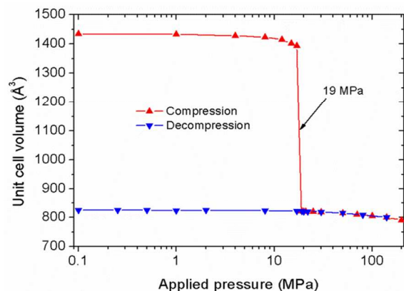
Fig. 3. MD simulated evolution of the unit cell volume of MIL-53(Al) at 300 K as a function of the applied pressure.
