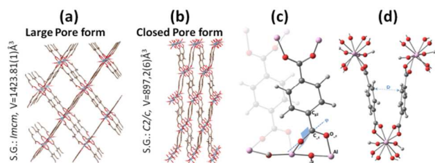
Fig. 1 Schematic representation of the pressure induced phase transition of the MIL-53(Al) between the large pore form (a) and the closed pore form (b). (c) and (d) provide an illustration of the Al-Oc-Cc-Cg 2 dihedral angle \phi and the mean distance D separating the phenyl rings respectively.
