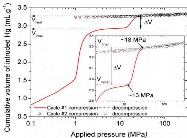
Fig. 2 Cumulative volume of intruded mercury in a two intrusion-extrusion cycles as a function of the applied pressure obtained for the MIL-53(Al) sample ( V_{\text{initial}} and V_{\text{final}} are the volumes of mercury intruded before and after the contraction of the solid respectively).
