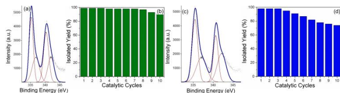
Fig. 3 (a, c) Pd 3d XPS spectra and (b, d) isolated yield of the product after recycling the catalysts up to 10 cycles for 0.41 wt% P-SiO 2 microcubes (a, b) and 0.37 wt% Pd NP – porous SiO 2 (c, d), respectively.
