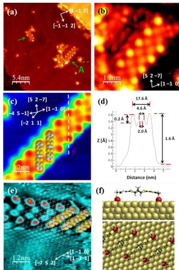
Fig. 3 STM images of TAT-TTF islands on Au(111) after annealing to 333 K (a) -0.6 V, 0.06 nA, 27 × 27 nm 2 (b) Island A, -0.6 V, 0.06 nA, 6 × 6 nm 2 (c) -0.9 V, 0.08 nA, 6 × 6 nm 2 (d) Line profile taken along white line indicated in (c). (e) -0.2 V, 0.13 nA, 6 × 6 nm 2 (f) Optimised DFT geometry of TAT-TTF bound via gold adatoms (red) to surface atoms (dark yellow).
