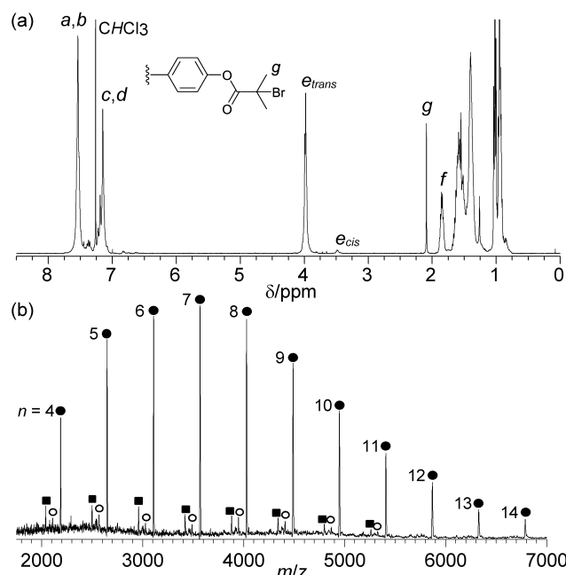
Fig. 1. (a) ^1\text{H} NMR spectrum of polymer 4b , (b) MALDI-TOF-mass spectrum of polymer 4b ( x_n indicated).
