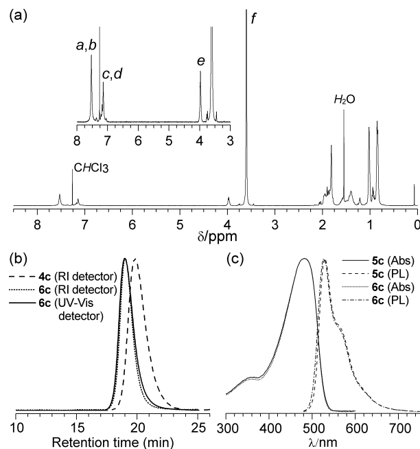
Fig. 2. (a) 1 H NMR spectrum of polymer 6c , (b) GPC chromatograms of polymer 4c and diblock copolymer 6c , (c) UV-Vis absorption and PL spectra of diblock copolymer 6c and the corresponding homopolymer 5c .
