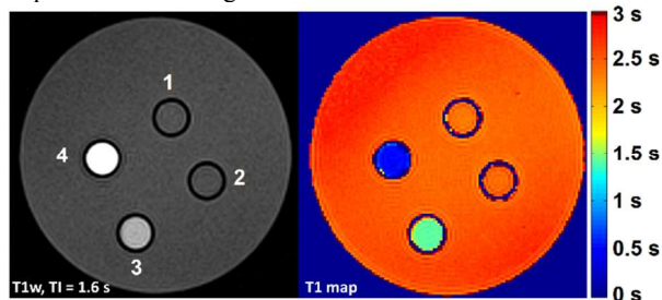
Fig. 6 MR images of 4 different solutions: 1. 4 (2 mM in water), 2. water, 3. water + 20 % piperidine and 4. 4 (2 mM in water + 20 % piperidine). For details see supporting information.
