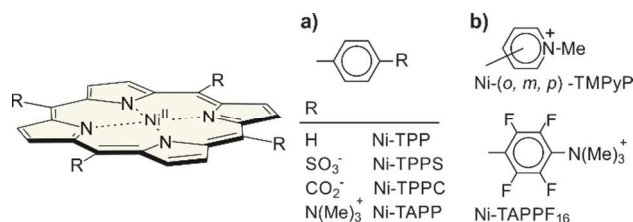
Fig. 1 Ni-tetraphenylporphyrin TPP and some water soluble derivatives. a) Electron rich porphyrins which do not bind axial ligands in water (diamagnetic). b) Electron deficient porphyrins which bind water (partially paramagnetic in water).
