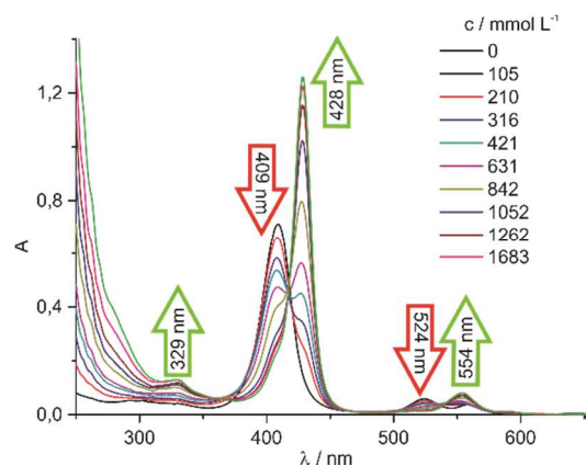
Fig. 3 UV-Vis spectra (top) of titration series of piperidine to Ni-porphyrin 4 (4.05 \mu M , 20 °C) in water. Association constants for addition of one piperidine ligand ( K_1 = 0.48 \text{ L mol}^{-1} ), and the association of a second piperidine ligand ( K_2 = 14.7 \text{ L mol}^{-1} ) were determined from the UV-visible data (see ESI). The green arrows correspond to increasing absorption upon increasing piperidine concentration.
