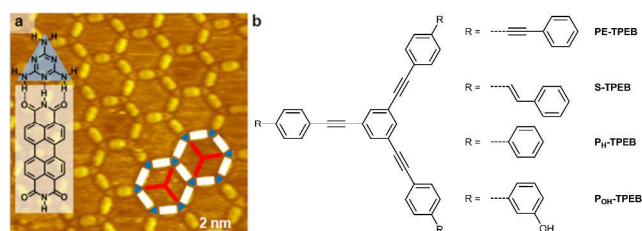
Fig. 1 (a) Melamine (blue triangle) and PTCDI (white rectangle) forming a triple hydrogen bonded honeycomb network as shown in the STM image. (b) Structures of the molecules investigated to sub-divide pores as illustrated in (a) with the red stars representing energetically equivalent positions of the molecules.
