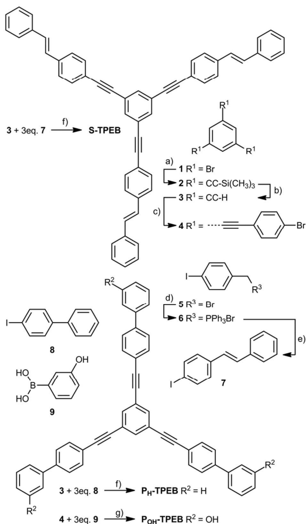
Scheme 1. Synthesis of the molecular stars S-TPEB , P H -TPEB and P OH -TPEB . Reagents and conditions: a) TMSA, Pd(PPh 3 ) 2 Cl 2 , CuI, THF, i Pr 2 NH, 60°C, 16h, quant.; b) K 2 CO 3 , THF, MeOH, r.t., 6h, quant.; c) IC 6 H 4 Br, Pd(PPh 3 ) 2 Cl 2 , CuI, THF, i Pr 2 NH, r.t., 5h, 79%; d) PPh 3 , DMF, 85°C, 1h, 76%; e) 1.) toluene, 0°C, t BuOK, C 6 H 5 CHO, r.t., 16h, CC; 2.) toluene, cat. I 2 , r.f.l., 3h, 77%; f) Pd(PPh 3 ) 4 , CuI, THF, i Pr 2 NH, r.t., 16h, 49% for S-TPEB , 83% for P H -TPEB ; g) Pd(PPh 3 ) 4 , K 2 CO 3 , toluene, EtOH, micro wave 120°C, 45min., 10%.
