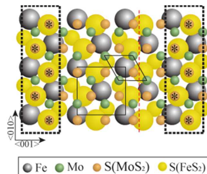
Fig. 4 Approximate lattice match obtained by laying \text{MoS}_2\{0001\} surface structure on top of \text{FeS}_2\{100\} at the orientations determined by the LEED patterns in figure 2. The matching S positions are highlighted within the dotted rectangles. The unit meshes for \text{MoS}_2\{0001\} and \text{FeS}_2\{100\} are noted as diamonds and squares, respectively. Only S atoms above the Fe layer in the \text{FeS}_2\{100\} surface are shown. \text{FeS}_2 glide plane is shown by red dashed line.
