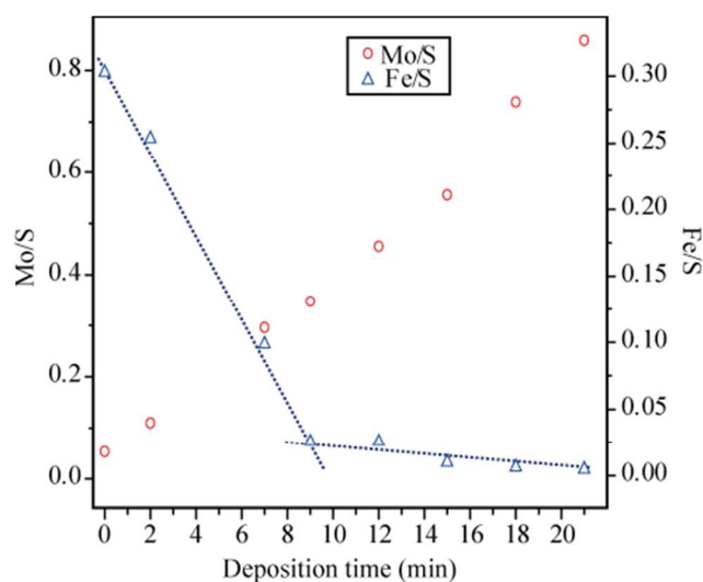
Fig. 1 Mo/S and Fe/S Auger peak height ratios (measured for the Mo peak at 190 eV kinetic energy, the Fe peak at 50 eV and the S peak at 155 eV) as a function of Mo deposition time on FeS 2 {100} surface (substrate was flash-annealed to 600K between successive deposition steps).
