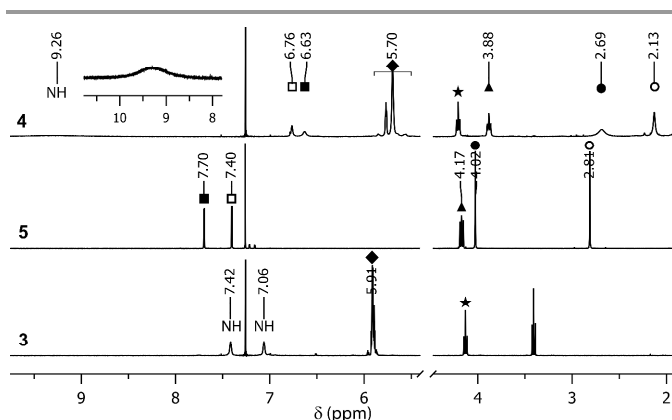
Fig. 2 Partial ^1\text{H} -NMR spectra of compounds 3 , 4 , and 5 recorded at 7 mM in \text{CDCl}_3 . Peak labels: Imidazolium -\text{CH}_3 (● and ○) and -\text{CH} peaks (■ and □); alkyl -\text{CH}_2 (▲); pyrrole -\text{CH} (◆); ester -\text{CH}_2 (★).
