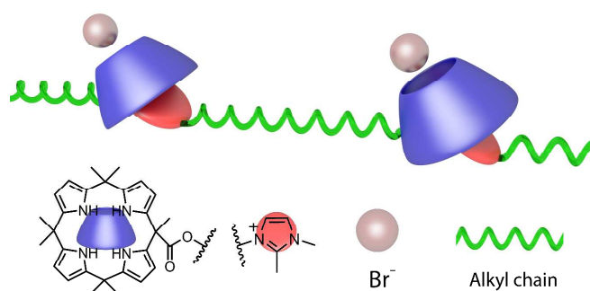
Fig. 1 Representation of the supramolecular polymer formed via the self-assembly of 4 .
