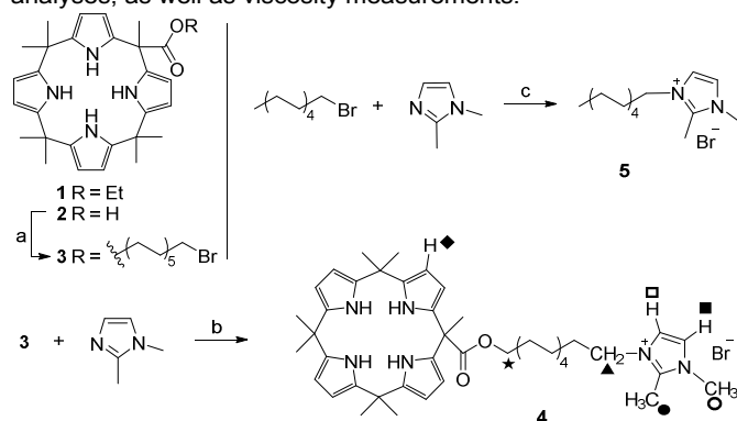
Scheme 1 Synthesis of imidazolium-functionalized calix[4]pyrrole and control compounds. Reagents and conditions: a) 11-bromo-1-undecanol, DCC/DMAP, \text{CH}_2\text{Cl}_2 , r.t.; b) \text{CH}_3\text{CN} , 70^\circ\text{C} , 24 h; c) n-propanol, reflux, 24 h.
