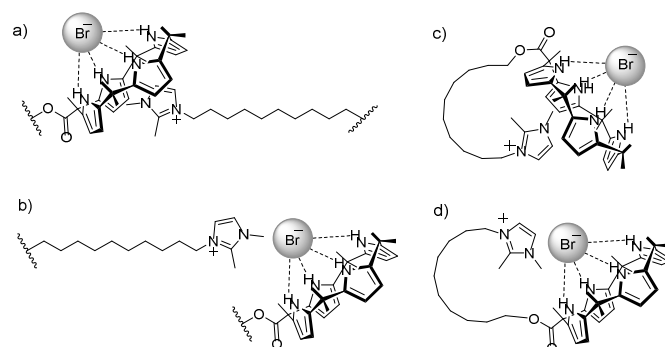
Fig. 3 (a) Schematic representation of the supramolecular polymer formed via the self-assembly of 4 . Also shown (b-d) are other possible binding modes for the imidazolium cation present in 4 .
