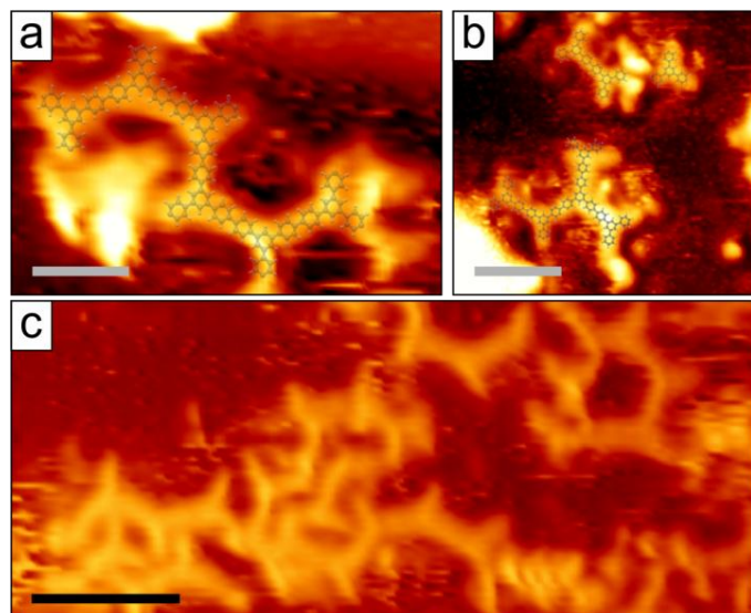
Figure 3 Oligomers of TBB on graphene/Ni(111). (a) High-resolution STM image of a hexamer with a superimposed scaled ball-and-stick model ( U_{\text{bias}} = -1.3 V, I = 32 pA). Scale bar: 1.5 nm. (b) High-resolution STM image of oligomers. ( U_{\text{bias}} = -0.8 V, I = 55 pA). Scale bar: 2.6 nm. (c) Overview STM image of reaction products. Oligomers of different sizes are visible with a lack of long-range order ( U_{\text{bias}} = -1.3 V, I = 32 pA). Scale bar: 3.3 nm.
