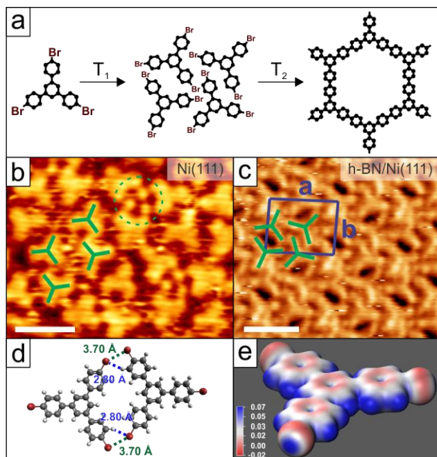
Figure 1 Structure of TBB and its adsorption on Ni(111) and h-BN/Ni(111). (a) Scheme of TBB (left) in the reaction from self-assembled structure (middle) to covalently connected oligomer (right). (b) High-resolution STM image of TBB on Ni(111). The molecules order locally with an absence of long-range order ( U_{\text{bias}} = -1.4 V, I = 52 pA). (c) High-resolution STM image of TBB self-assembled on h-BN/Ni(111) ( U_{\text{bias}} = -0.8 V, I = 50 pA). Scale bar in b and c: 2.0 nm. (d) Calculated dimer as observed in the self-assembled network with stabilizing close contacts between Br and H atoms. (e) Electrostatic potential map of TBB monomer. Units in Rydberg/e.
