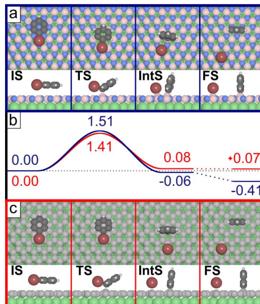
Figure 4 Initial state (IS), transition state (TS), intermediate state (IntS) and final state (FS) of the dehalogenation of bromobenzene on (a) h-BN/Ni(111) and (c) graphene/Ni(111). (b) Energy diagram of the reaction on h-BN/Ni(111) in blue and on graphene/Ni(111) in red. Both substrates exhibit a barrier of approximately 1.5 eV for the debromination. (Grey: carbon, white: hydrogen, brown: bromine, blue: nitrogen, light pink: boron, green: nickel). Values in eV.
