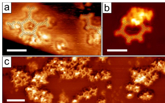
Figure 2 Reaction products of TBB on h-BN/Ni(111). (a) High-resolution STM image of a pentagon-shaped oligomer (left) and a trimer (right). Scaled ball-and-stick models are superimposed ( U_{\text{bias}} = -1.0 V, I = 46 pA). (b) High-resolution STM image of a quasi-hexagon ( U_{\text{bias}} = -1.5 V, I = 330 pA). (c)
