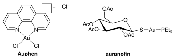
Fig. 1. Gold complexes used in this study.
