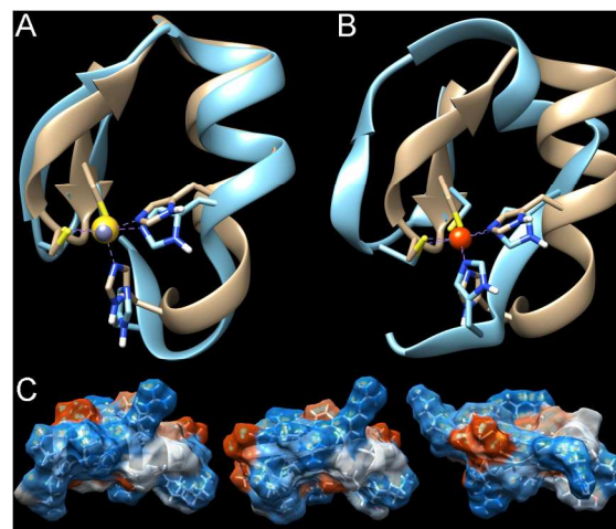
Fig. 4. A) Overlap between the calculated structures of 2a (brown) and 3a (light blue). B) Overlap between the calculated structures of 2a (brown) and 4a (light blue). C) Hydrophobicity surfaces of 2a (left), 3a (middle) and 4a (right).
