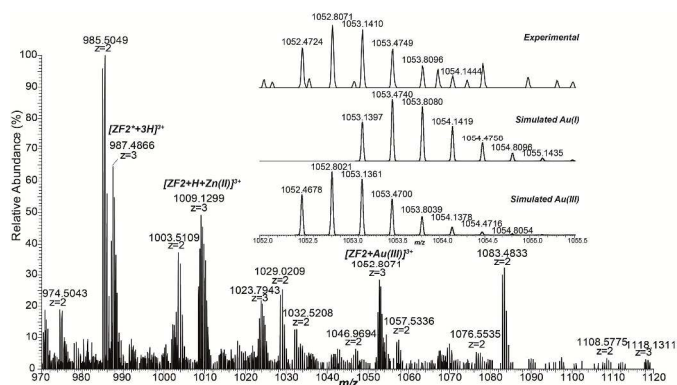
Fig. 2. ESI Orbitrap FT-MS mass spectrum of the ZF2-Auphen adduct recorded after 5 min incubation with Zn 2+ followed by 15 min incubation with Auphen. The insets compare the experimental isotopic pattern of peptide-metal complex with the simulated isotopic patterns of the (C 127 H 203 N 39 O 39 S 2 Au(I)) 3+ and (C 127 H 201 N 39 O 39 S 2 Au(III)) 3+ composition peptides.
