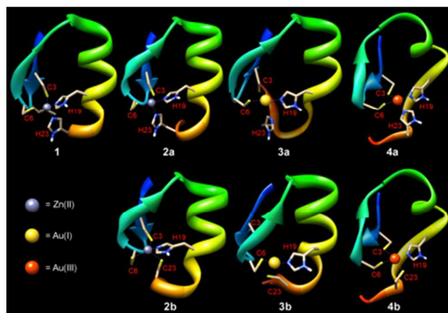
Fig. 3. NMR structure ( 1 ) of the 31 st zinc finger from the Xenopus protein Xfin (Xfin-31, pdb code 1ZNF) compared to the optimized QM/MM structures obtained from the Xfin31 Cys 2 His 2 peptide ( 2a–4a ) and its Cys 2 HisCys analogue ( 2b–4b ). Structure and colour code: coordination sphere a = Cys 2 His 2 , b = Cys 2 HisCys; 1 and 2 = Zn(II) (Grey), 3 = Au(I) (Yellow) and 4 = Au(III) (Orange).
