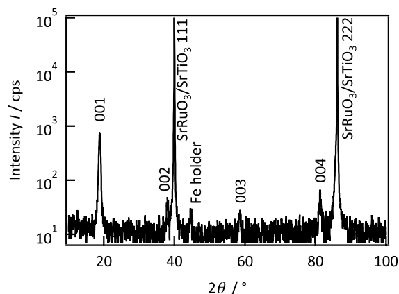
Fig. 1 Out-of-plane XRD pattern for a \text{Li}_2\text{MnO}_3 film on \text{SrRuO}_3(111)/\text{Nb}:\text{SrTiO}_3(111) .
