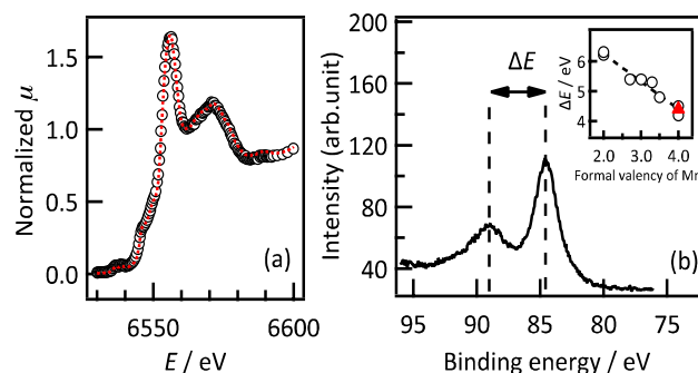
Fig. 2 (a) Mn-K edge XANES and (b) Mn 3s HAXPES spectrum of a \text{Li}_2\text{MnO}_3(001) film. The red dashed line in (a) depicts the XANES spectrum of polycrystalline \text{Li}_2\text{MnO}_3 . The inset of (b) shows the splitting width of the \text{LiMnO}_3(001) film (denoted as \blacktriangle ), polycrystalline \text{Mn}^{2+}\text{O} , \text{Mn}^{2.67+}_3\text{O}_4 , \text{LiMn}^{3+}\text{O}_2 , \text{La}_{0.9}\text{Mn}^{3.3+}\text{O}_3 , \text{La}_{0.5}\text{Ca}_{0.5}\text{Mn}^{3.5+}\text{O}_3 , \text{Li}_2\text{Mn}^{4+}\text{O}_3 , and \text{SrMn}^{4+}\text{O}_3 (denoted as \circ ) as a function of the formal Mn valency.
