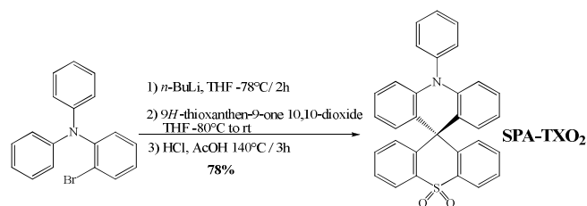
Scheme 1. Synthesis of SPA-TXO 2
