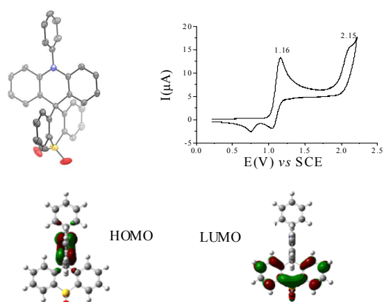
Fig 1. Top. ORTEP drawing (left, 50% ellipsoid probability) and cyclic voltammetry ( 100 \text{ mV}\cdot\text{s}^{-1} ) in \text{CH}_2\text{Cl}_2/[\text{NBu}_4][\text{PF}_6] 0.2M (right) of SPA-TXO 2 . Bottom: Calculated nature of the highest occupied (HOMO) and lowest unoccupied (LUMO) orbitals of SPA-TXO 2 (isovalue 0.04)
