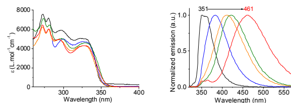
Fig 2. Absorption and Emission spectra of SPA-TXO 2 , \lambda_{\text{Exc}} = 300 \text{ nm} , in different solvents (cyclohexane: black line, toluene: blue line, chloroform: green line, ethyl acetate: orange line, acetonitrile: red line).
