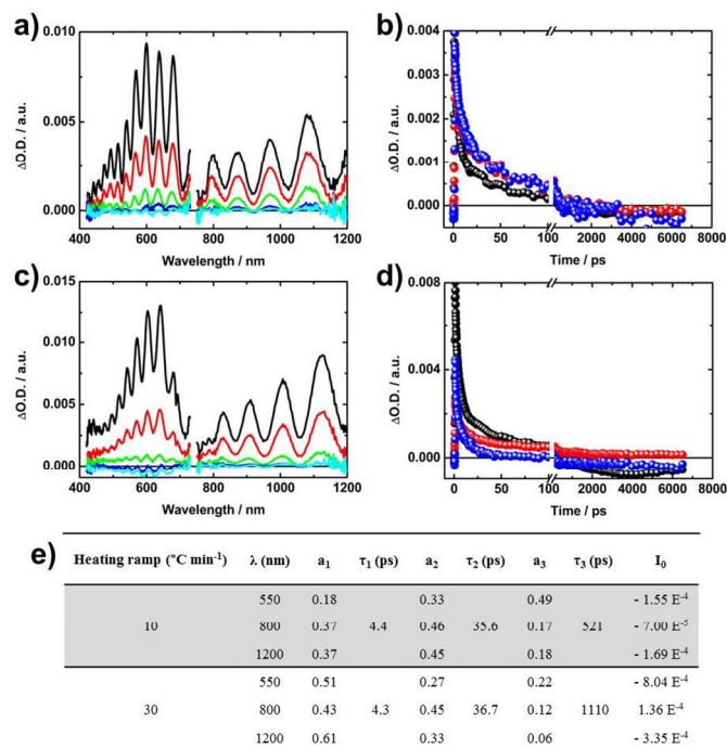
Figure 3 - a) and c) Differential absorption spectra (visible and near-infrared) measured by femtosecond flash photolysis (258 nm) at different time delays of 1 ps (black), 10 ps (red), 100 ps (green), 1000 ps (blue), and 6500 ps (cyan); b) and d) Relative absorption time profiles of the spectra a) and c) at 550 nm (black), 800 nm (red) and 1200 nm (blue) corresponding to absorption of holes, trapped-electrons and free electron, respectively. Data in a), b), c) and d) were measured for ca. 3 \mu m-thick TiO 2 nanotube layers (grown on quartz slides) that were annealed at 500 °C with heating rate of a), b) 10 °C min -1 and a), b) 30 °C min -1 ; e) data obtained by fitting the decay transient curves to three exponential functions (at 550, 800 and 1250 nm) in order to distinguish the contributions of the different transient species ( i.e. , holes, trapped-electrons and free electron).
