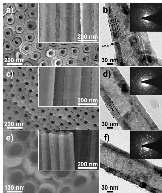
Figure 2 - High-magnification top view SEM images of TiO 2 nanotube membranes annealed in air at 500 °C by using heating rate of a) 10, c) 30 and e) 60 °C min -1 . The images were taken at middle height along the length of the tubes after cracking the anodic layers. Insets: relative high-magnification cross-sectional SEM images of the nanotubes; TEM images of tubes annealed in air at 500 °C by using heating rate of b) 10, d) 30 and f) 60 °C min -1 . Insets: relative SAED patterns showing the typical reflections of TiO 2 anatase phase.
