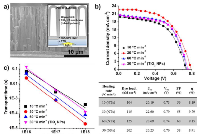
Figure 1 - a) Cross-sectional SEM image of a photo-anode consisting of a 20 μm-thick TiO 2 NT membrane that was fabricated by the re-anodization approach and transferred in tube-top-down configuration on a FTO slide coated with a 2 μm-thick TiO 2 NP film. Inset: a sketch of the photo-anode configuration adopted for assembling the DSSCs; b) J-V curves and a summary of the photovoltaic characteristics of the different DSSCs measured under simulated AM 1.5 front-side illumination; c) IMPS measurements performed on the different DSSCs (the continuous lines are a guide to the eye).
