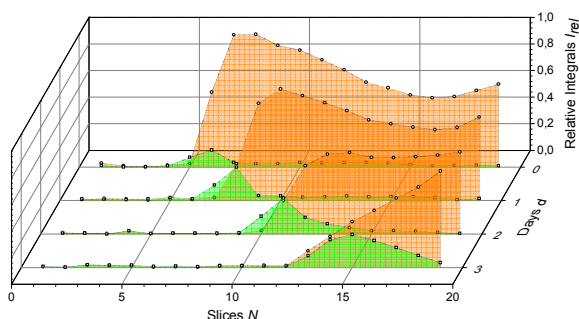
Figure 3. Relative integrals for the ^1\text{H} NMR signals at -0.59 ppm (green) and that of the n\text{BuLi} \alpha\text{-CH}_2 protons (orange) as function of the slice number, 3 h, 1, 2 and 3 days after addition of PMDTA to n\text{BuLi} inside the pre-swollen polystyrene gel. All signals high-field to -0.59 ppm were attributed to “ n\text{BuLi} ”.
