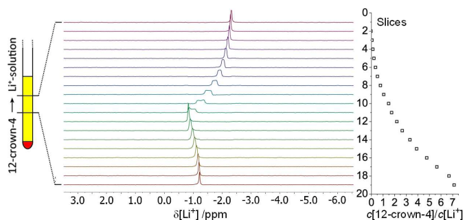
Figure 1. Slice-selective 7 Li NMR spectra of LiClO 4 in acetonitrile- d 3 in the presence of a concentration gradient of 12-crown-4, 6 h after sample preparation. Generally, slices (1 mm thick, 1 mm distance each) are numbered from the top of the active volume to the bottom, with slice 10 located at the centre. The 12-crown-4/LiClO 4 concentration ratio is indicated on the right and increases from slice 1 to slice 19.
