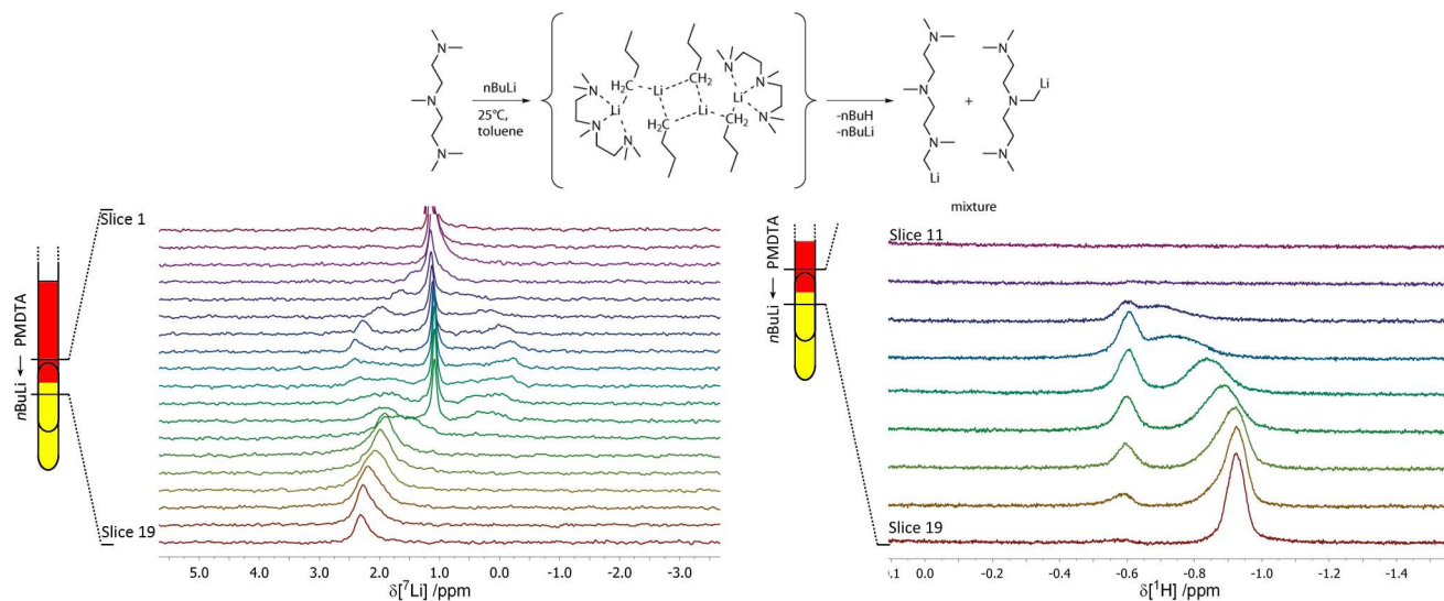
Figure 2. Top: The reaction between n\text{BuLi} and PMDTA yields lithiated PMDTA via the intermediate [(n\text{BuLi})_2\text{PMDTA}]_2 . Bottom left: Slice-selective ^7\text{Li} NMR spectra (slices 1 to 19) of the reaction within a polystyrene gel, 3 days after the addition of PMDTA. Bottom right: Slice-selective ^1\text{H} NMR spectra (slices 11 to 19) of the same sample.
