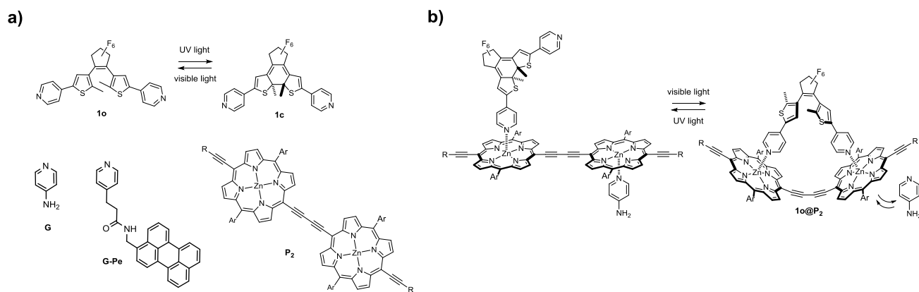
Fig. 1 a) Isomerization scheme of 1 and molecular structures of 4-aminopyridine ( G ), the perylene functionalized analog ( G-Pe ), and the porphyrin dimer ( P 2 ). b) Photo-release principle. Ar = Si(C 6 H 13 ) 3 , R = 3,5-di( tert -butyl)phenyl.
