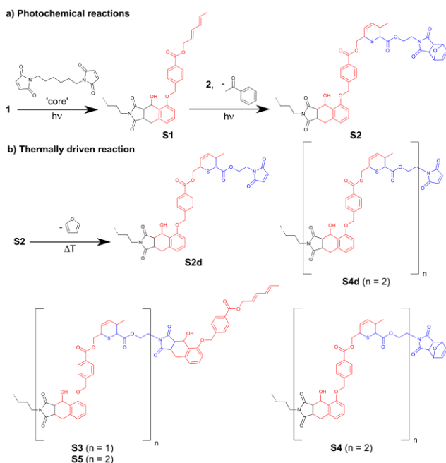
Fig. 1. Synthetic pathway for the photochemical construction (a) of the sequence defined polymer and intermediate retro-Diels–Alder (rDA) deprotection (b). For clarity, only one part of the synthesized symmetrical molecules is represented.
