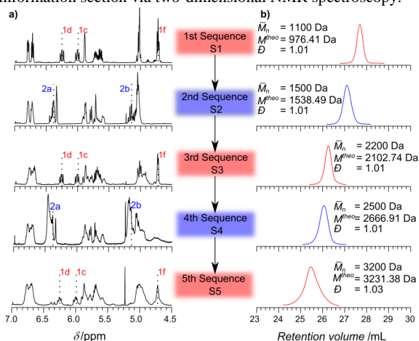
Fig. 3. Evolution of ^1\text{H} Nuclear Magnetic Resonance (NMR) spectra (a) and Size Exclusion Chromatography (SEC) traces (b) of the sequence defined products S1 to S5 . (a) The NMR resonance of the key protons of synthon 1 ( 1c , 1d and 1f ) and 2 ( 2a and 2b ) are shown (500 MHz, \text{CDCl}_3 ). (b) SEC performed in THF (PS calibration).
