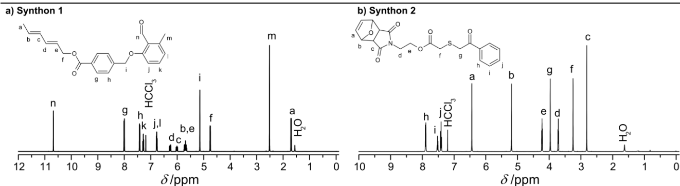
Fig. 2. ^1\text{H} Nuclear Magnetic Resonance (NMR) spectra of the two hetero bifunctional photoreactive monomers 1 (a) and 2 (b) (500 MHz, \text{CDCl}_3 ).
