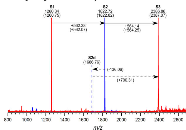
Fig. 4. Electrospray ionization mass spectra (ESI-MS) of the sequence products S1 to S3 (theoretical values in brackets). For clarity, the theoretical peak for S2d is provided (see text).
