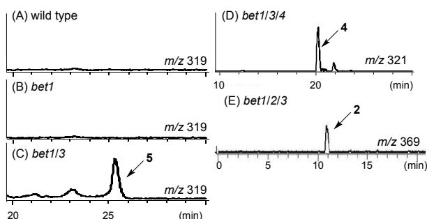
Figure 2. LC-MS profiles of metabolites produced by transformants. A) A. oryzae NSAR1. B) bet1 transformant. C) bet1/3 transformant. D) bet1/3/4 transformant. E) bet1/2/3 transformant.
