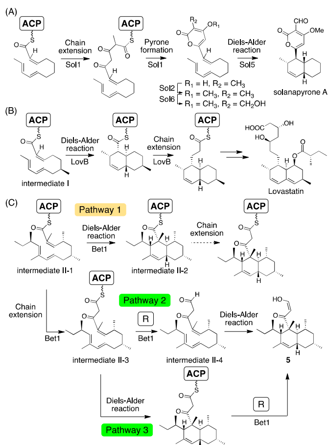
Scheme 2. Proposed mechanism of decalin scaffold formation in (A) solanapyrone A, (B) lovastatin, and (C) betaenone biosynthesis.
