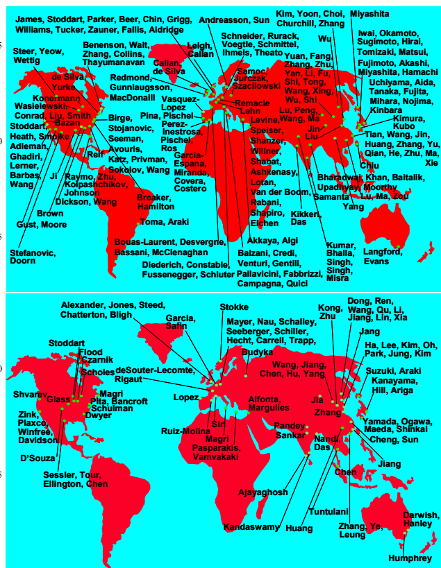
Figure 1a and 1b. Approximate world maps of the sources of molecular logic devices. Single input - single output devices have been omitted.
