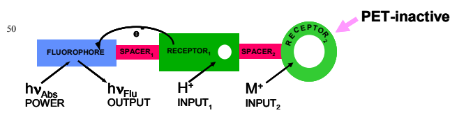
Figure 4. 'Fluorophore-spacer 1 -receptor 1 -spacer 2 -receptor 2 ' system exemplified by 1.
