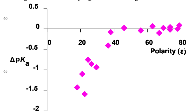
Figure 6. Effective local H + density (as measured by the shift of acidity constant relative to bulk water, \Delta pK_a ) as a function of position of 7 (as measured by the local dielectric constant, \epsilon ) within an aqueous micelle solution of Triton X-100. Plotted from data in ref. 79.
