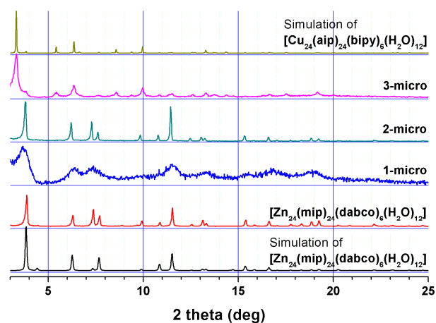
Fig. 3 Comparison of the PXRD patterns of 1-micro , 2-micro and 3-micro with those of [Zn 24 (mip) 24 (dabco) 6 (H 2 O) 12 ] 22 and [Cu 24 (aip) 24 (bipy) 6 (H 2 O) 12 ] 23 .
