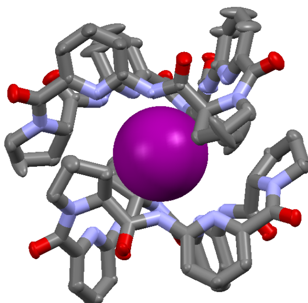
Figure 2. X - ray crystal structure of the 2:1 ‘sandwich complex’ formed between 18 and iodide. Figure generated from X-ray diffraction data originally published in reference 47.
