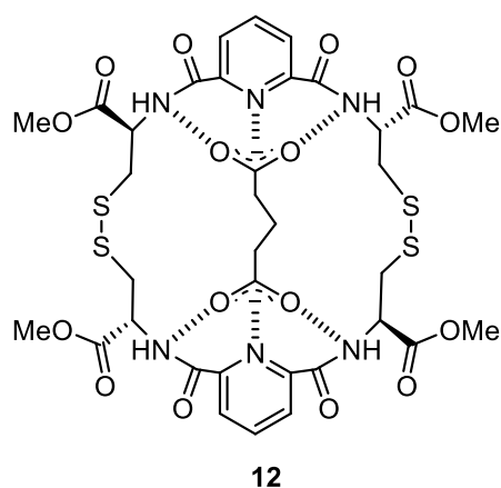
Figure 1: The proposed tetrahydrogen – bonded structure for the molecular recognition of 12 and glutaric acid
