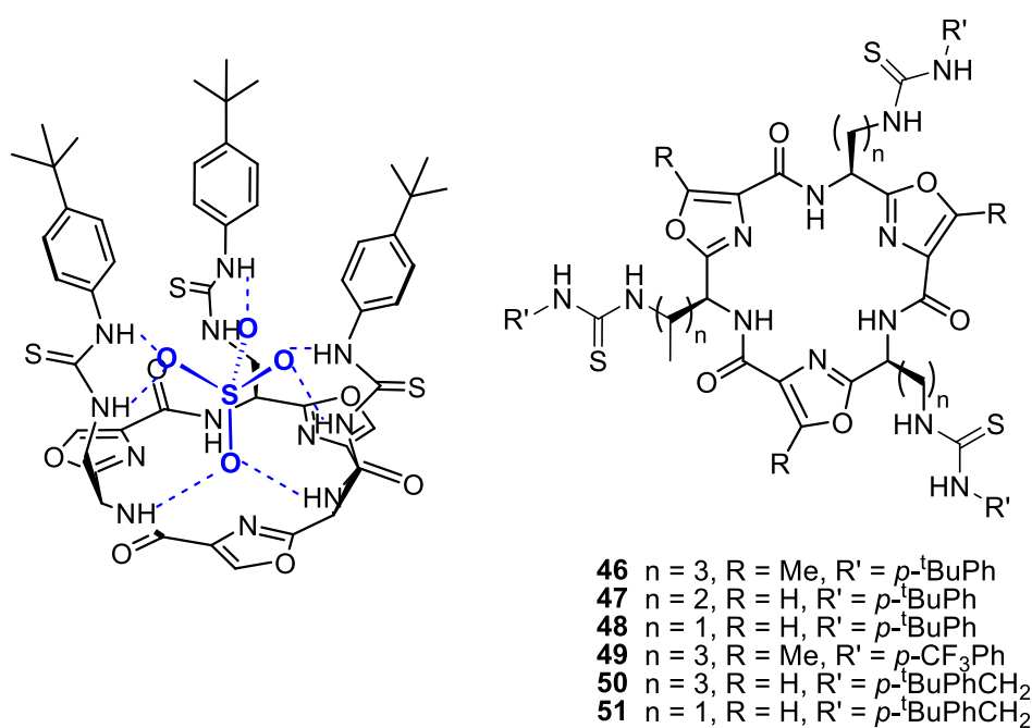
Figure 9. Proposed binding mode between 48 and sulfate and structures of compounds 46-51 .
