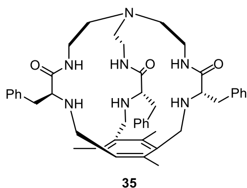
Figure 7. General structure of the pseudopeptidic tripodal cages.
