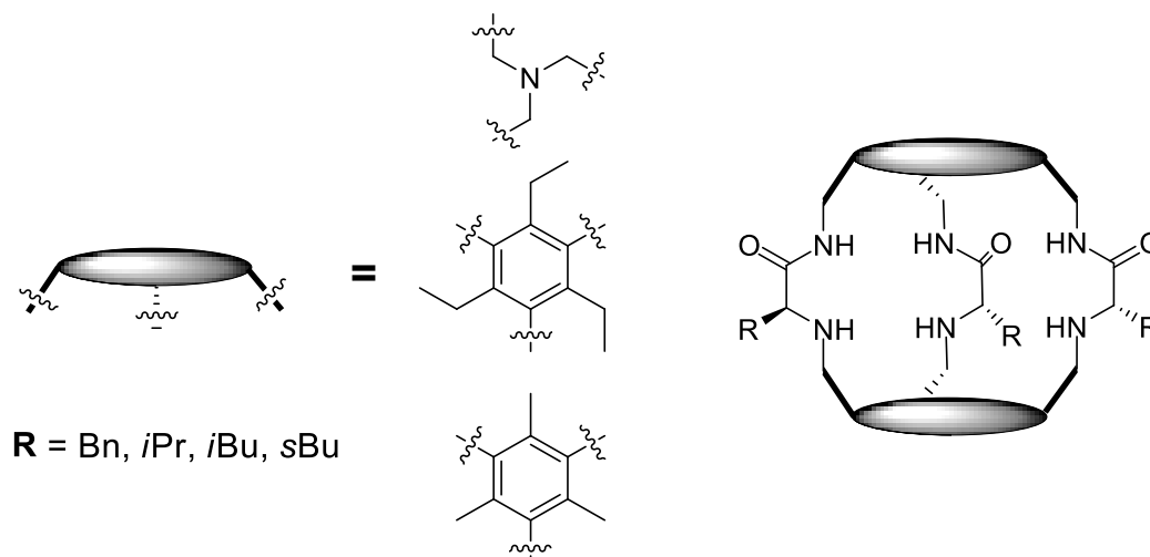
Figure 7. General structure of the pseudopeptidic tripodal cages.
