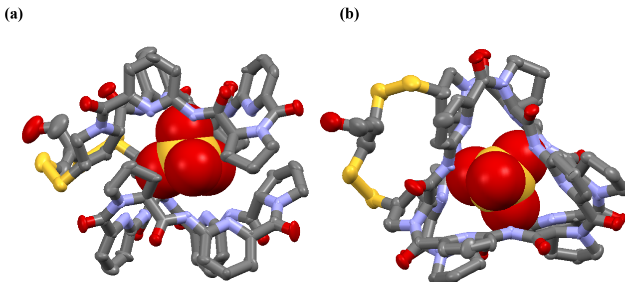
Figure 5. X - ray crystal structure of the 1:1 ‘sandwich complex’ formed between 23 and sulfate (a) viewed from the side and (b) viewed from above. Figure generated from X-ray diffraction data originally published in reference 52.
