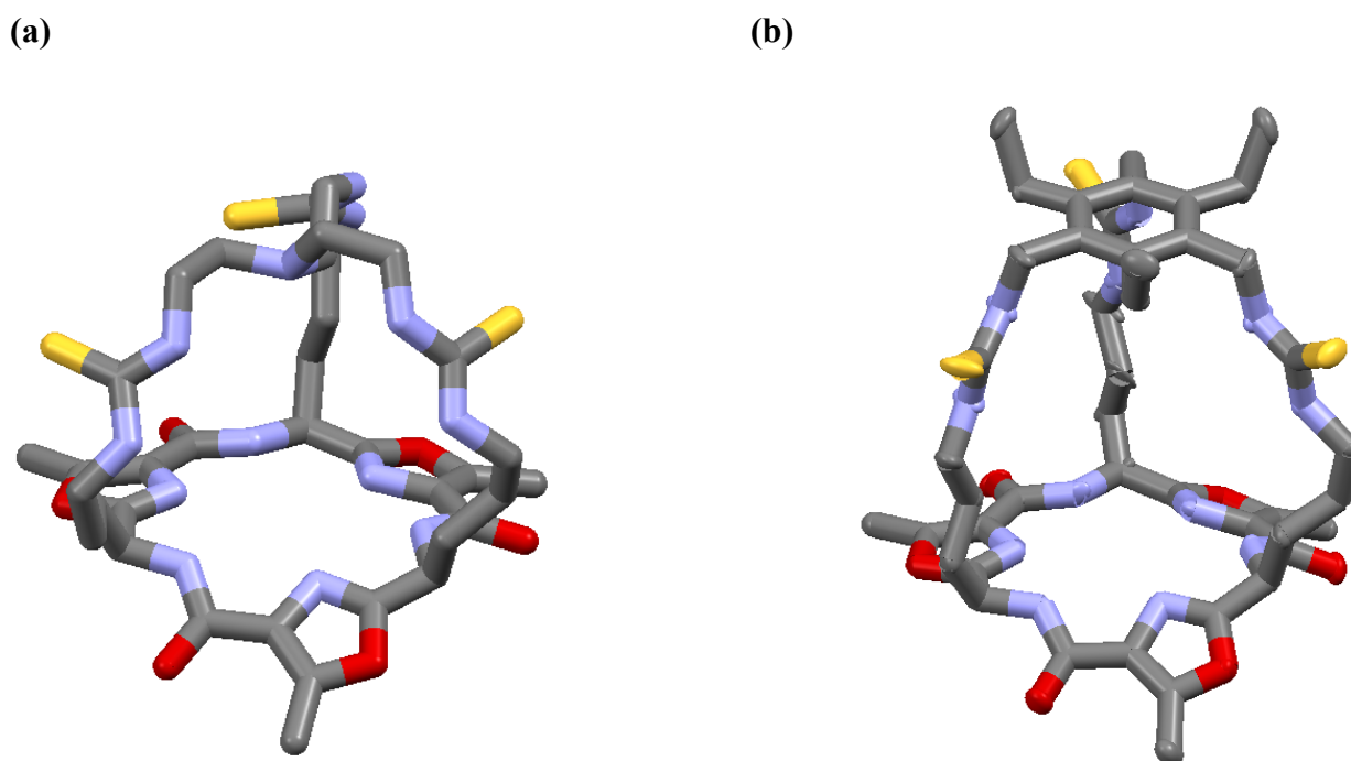
Figure 10. X - ray crystal structures of (a) 52 and (b) 53 . Solvent molecules have been removed for clarity. Figure generated from X-ray diffraction data originally published in reference 79.
