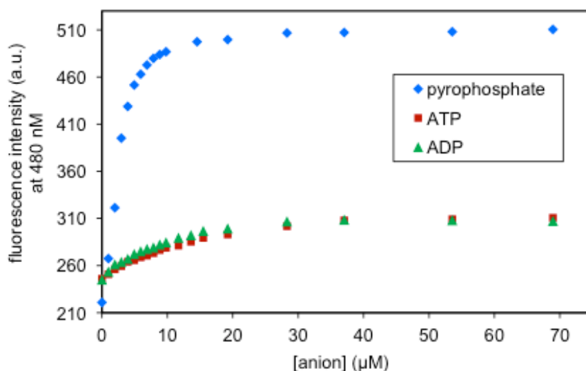
Figure 12. A comparison of the changes in fluorescence emission observed for the complex formed between a coumarin methylsulfonate indicator and 69 (10 mM) upon the addition of various anions in Krebs buffer solution.
