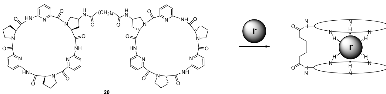
Figure 3. Complexation of iodide by a molecular ‘oyster’.
