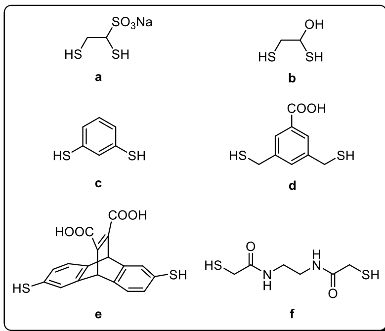
Figure 4. The six dithiols of varying length and rigidity used to optimise the linking unit between two Apa-based cyclic peptides.
