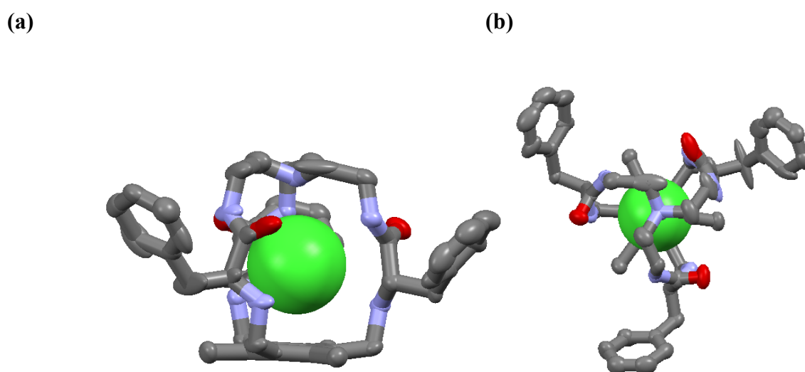
Figure 8. Side (a) and upper (b) views of the crystal structure of the [35·4Cl] salt with the chloride anion clearly shown binding inside the macrocyclic cavity. Externally bound chloride anions, crystallization water molecules and hydrogens have been omitted for clarity. Figure generated from X-ray diffraction data originally published in reference 63.
