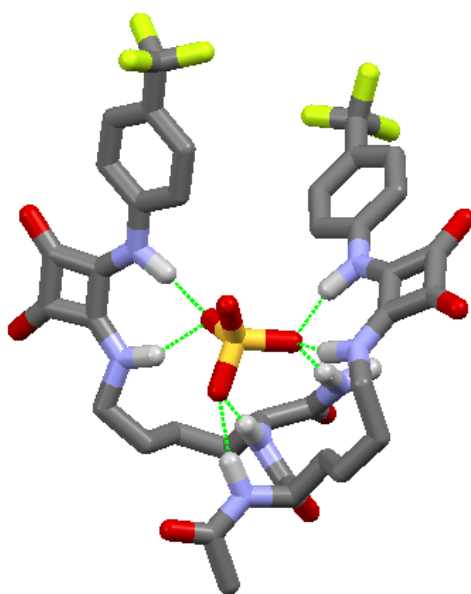
Figure 11. DFT calculated structure of the \text{SO}_4^{2-} complex of 60 showing sulfate inserted into the binding cavity stabilised by 7 N-H...O hydrogen-bond interactions.
