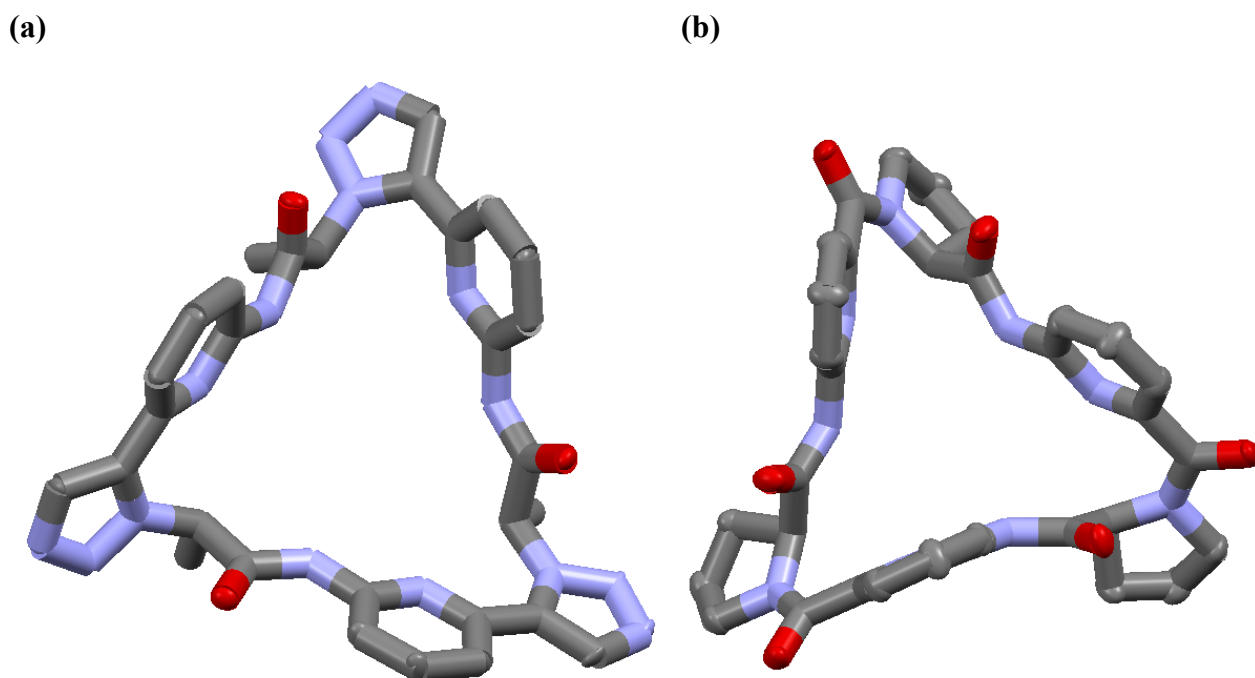
Figure 6. Comparison of the X - ray crystal structures of (a) 32 and (b) 18 . Figure generated from X-ray diffraction data originally published in references 58 and 47.
