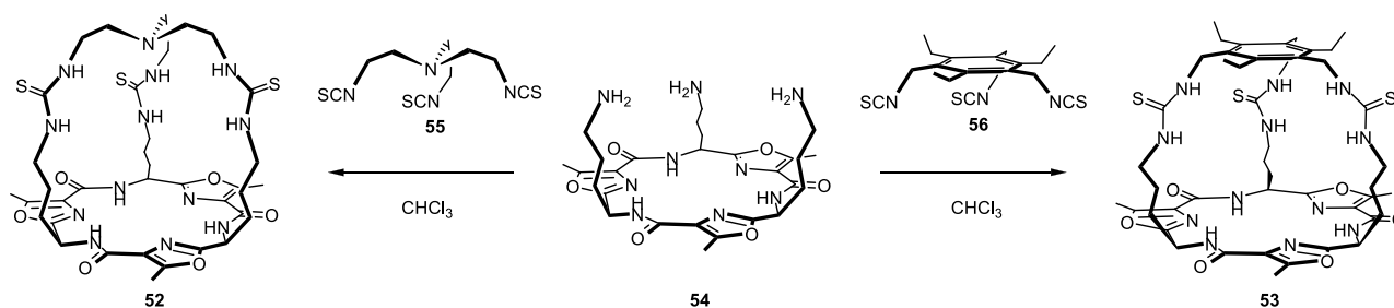
Scheme 1. General synthetic approach to cyclic peptide based cryptands 52 and 53 .
