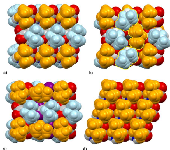
Fig. 9. (a) Space-filling representation of one face of a molecular layer of NiPrV. (b) Similar representation for NiPrVR. The hydrophobic groups that have been interchanged compared to NiPrV have been highlighted. (c) Molecular layer of NiPrL. (d) Hydrophobic surface in the crystal structure of DL-Val.
