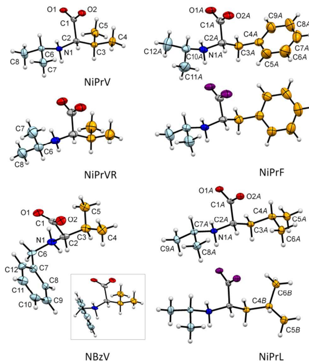
Fig. 3. Molecular structures of NiPrV, NiPrVR, NiPrL, NiPrF and NBzV. Displacement ellipsoids are shown at the 50% probability level. Side chains are colored in orange, N-alkyl groups in light blue. For structures with Z = 2 the two molecules are distinguished by carboxylate O atoms being violet for molecule B. To facilitate comparison with NiPrV, a molecule with L-configuration is shown for NiPrVR. Atomic labels have been omitted when they are identical to the ones in the molecule above. The small, framed illustration for NBzV shows the molecule in an orientation similar to the other compounds.
