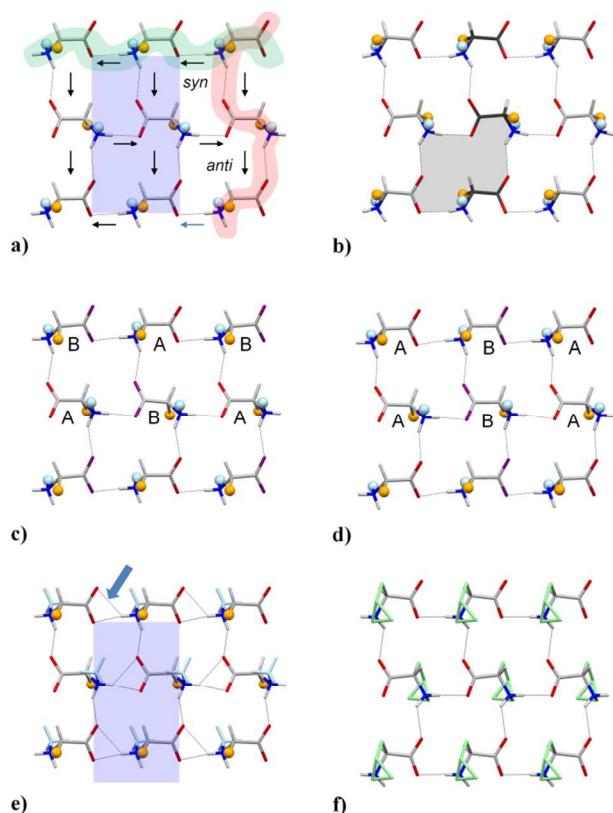
Fig. 6. Hydrogen-bonded sheets in (a) NiPrV, (b) NiPrVR, (c) NiPrF, (d) NiPrL, (e) WAJBIS 6 and (f) GEVMOK. 11 Hydrogen bonds shorter than 2.6 Å are indicated by dotted lines. The weaker component in the three-center interaction indicated for WAJBIS (arrow) is 2.46 Å (after normalization of the N-H distance to 0.92 Å). In other structures the corresponding distances are > 2.67 Å. Two C(4) chains have been highlighted in (a), arrows indicate the directions of the N-H bond vectors. The blue shade gives the size of the repeating pattern of NiPrV (in this case equivalent to the footprint of the unit cell). The same shade (on the same scale) appears in (e). A R_4^4(16) ring system is shaded in (b).
