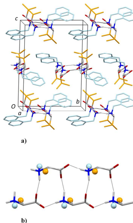
Fig. 7. (a) Unit cell and crystal packing of NBzV. (b) Hydrogen bonding pattern of NBzV. Color coding and style as in Fig. 4 and Fig. 5
