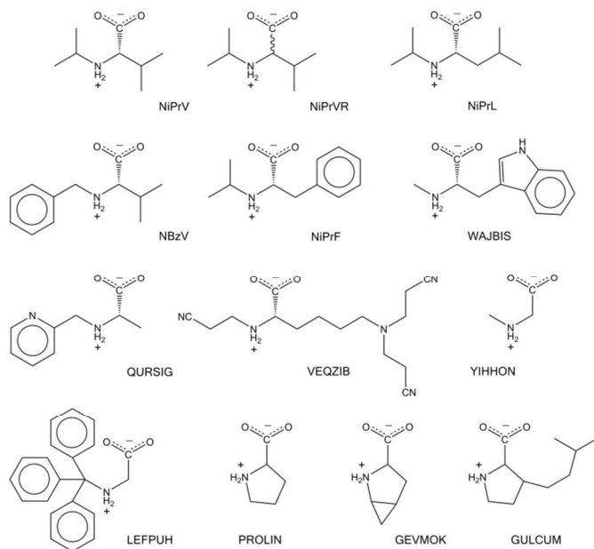
Fig. 2. N-alkylated amino acids discussed in this paper. Previously investigated molecules 5-12 have been identified by their CSD 4 reffcodes.
