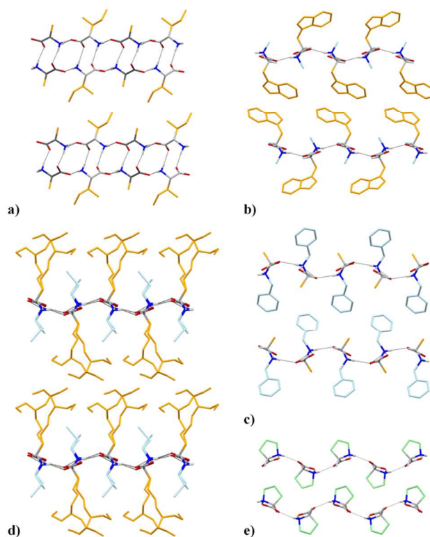
Fig. 8. Crystal packing of (a) L-Ile:D-Ala (FITHIZ), 16 (b) N -methyl-L-tryptophan (WAJBIS), 6 (c) N -(2-pyrimidylmethyl)-L-alanine (QURSIG), 7 N α , N ε , N ζ -tri(cyanoethyl)-L-lysine (VEQZIB), 8 and (e) L-proline (PROLIN). 10 Color coding as in Figure 3. The C-atoms in the ring system of L-proline appear in light green.
