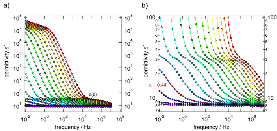
FIG. 6: a) real part of the complex permittivity \epsilon' of nanocrystalline \text{Ba}_{0.6}\text{La}_{0.4}\text{F}_{2.4} (sample 1) as a function of frequency \nu . b) magnification of the spectra shown left in order to estimate \epsilon(0) . The bulk process can be mirrored with a power law of the form \epsilon'(\nu) = \epsilon(\infty) + A_\epsilon \nu^{-p} with p \neq f(t) \approx 0.44 .
