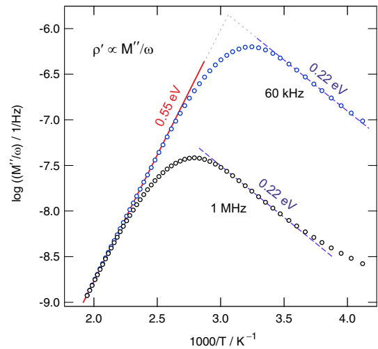
FIG. 9: real part of the complex resistivity of nanocrystalline \text{Ba}_{0.6}\text{La}_{0.4}\text{F}_{2.4} (sample 3) as a function of inverse temperature T . From the different flanks of asymmetric peaks obtained activation energies for long- and short-range motion can be deduced.
