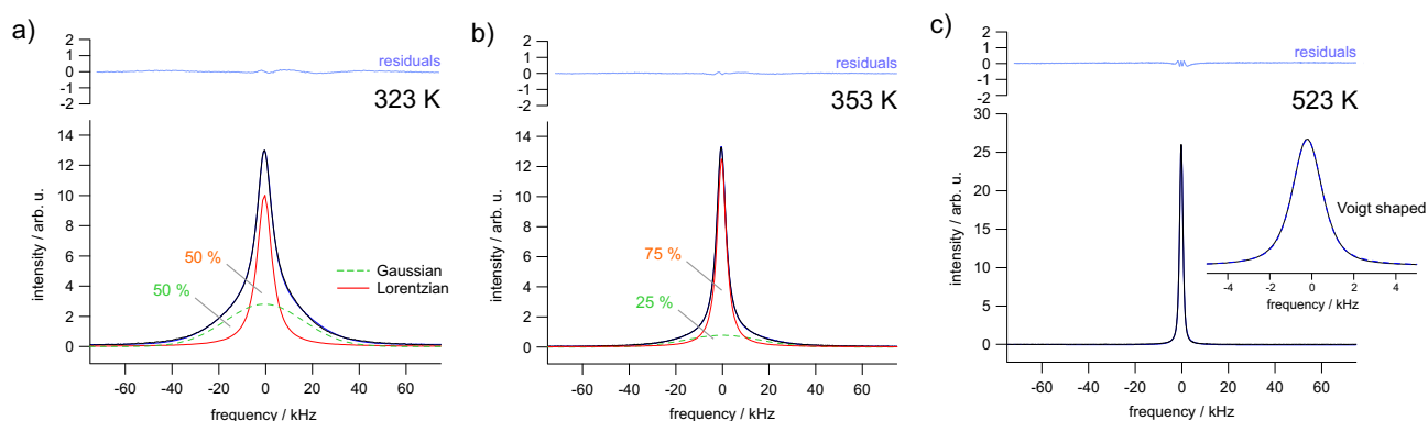
FIG. 4: Selected ^{19}\text{F} NMR lines to highlight the motional averaging of dipole-dipole interactions and coalescence as well. While a combination of a Gaussian and a Lorentzian is appropriate to represent the lines at moderate temperatures, the final shape in the regime of extreme narrowing resembles that of a Voigt function. The values in percentage terms indicate the area fractions of the two different components.
