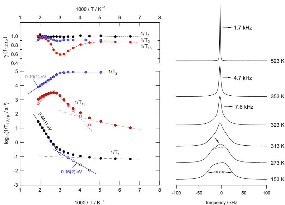
FIG. 3: Left: temperature dependence of the ^{19}\text{F} NMR relaxation rates of nanocrystalline \text{Ba}_{0.6}\text{La}_{0.4}\text{F}_{2.4} (sample 1) prepared by mechano-synthesis at ambient temperature. The Larmor frequency was 282 MHz. The upper graph shows the dependence of the stretching exponents \gamma on T . Right: ^{19}\text{F} NMR line shapes recorded under static conditions at the temperatures T indicated.
