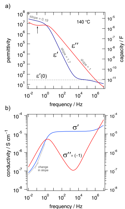
FIG. 7: a) the frequency dependence of \epsilon' and \epsilon'' recorded at 413 K. b) frequency dependence of \sigma' and (-1) \cdot \sigma'' recorded at 413 K. According to the Kramers-Kronig relation and \hat{\sigma}(\omega) = i\omega\epsilon_0\hat{\epsilon}(\omega) (here, we have \omega/2\pi = \nu , i^2 = -1 and \epsilon_0 being the permeability in the vacuum) the plateau \omega' \propto A_\sigma \nu^0 corresponds to \epsilon' \propto A_\epsilon \nu . The local minimum of \epsilon'' (see arrow) is expressed as a change in slope in the EP region of \sigma' , see also Fig. 5. The slopes given for \epsilon' indicate electrode polarisation.
