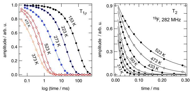
FIG. 2: Left: ^{19}\text{F} NMR transversal decay of the spin-locked magnetization recorded at the various temperatures indicated. The locking frequency was 62.5 kHz. Note the logarithmic scale of the x -axis. Solid lines represent fits according to stretched exponentials yielding T_{1\rho}^{-1} and \gamma_{1\rho} . Right: ^{19}\text{F} NMR spin-spin relaxation transients. From the fits (stretched exponentials, solid lines) the rates T_2^{-1} and stretching factors \gamma_2 shown in the upper part of the Arrhenius plot of Fig. 3 can be obtained. The corresponding T_1 -transients do almost follow an exponential time behaviour.
