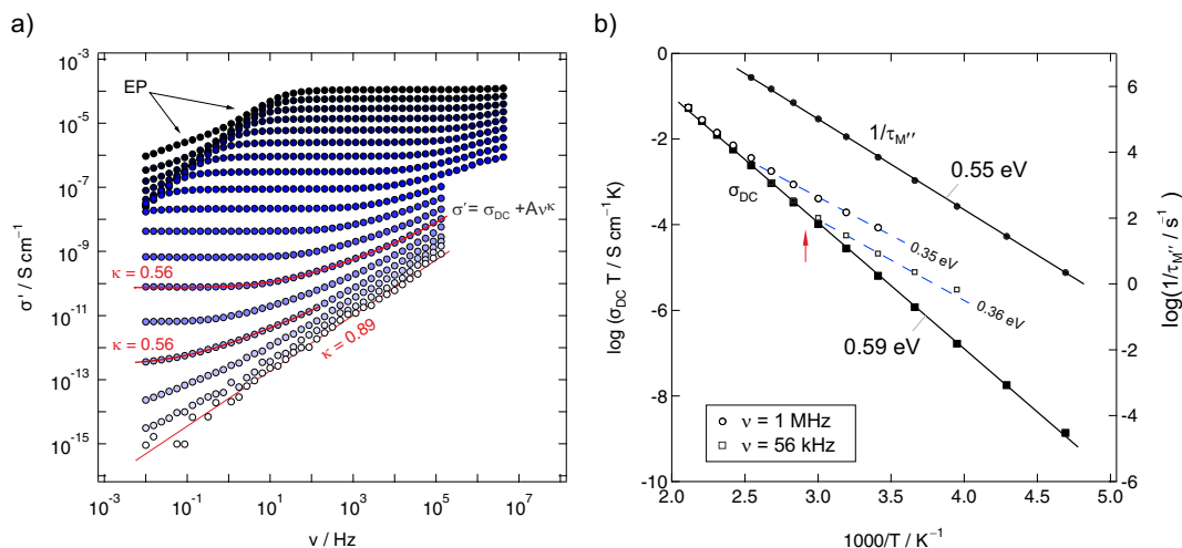
FIG. 5: a) impedance isotherms of mechanosynthesized \text{Ba}_{0.6}\text{La}_{0.4}\text{F}_{2.4} (sample 1) recorded at temperatures ranging from 133 K up to 473 K. b) Arrhenius plot of \sigma_{\text{DC}}T ; for comparison, the temperature dependencies of \sigma'T , read out at frequencies \nu = 1 MHz and 56 kHz, respectively, are also shown. Moreover, \tau_{M''}^{-1} , that is the relaxation rate being determined from modulus spectra M''(\nu) , is also presented.
