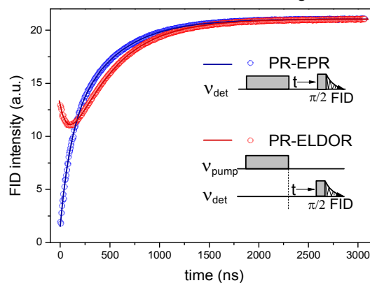
Fig. 3 Recovery curves and fits of the FID in EPR and ELDOR polarization recovery measurements on 1.6 mM TEMPONE-D- ^{15}\text{N} in toluene. Experimental set up and conditions are similar to Fig. 2.
