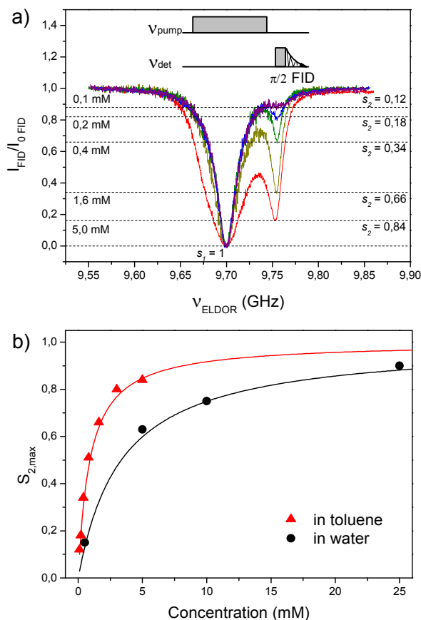
Fig. 2 a) EPR FID intensity of the high-field hf line of TEMPONE-D- ^{15}\text{N} as a function of the frequency of the saturating (pump) pulse. Exp. details: detection is 30 MHz off resonance on the high field side to minimize simultaneous excitation of the low field line; t(\pi/2) = 16 ns; t(\text{pump}) = 1 \mu\text{s} . B_1 \sim 2\text{-}3 G. Error due to ringing was \leq 10\% . b) Concentration dependence of s_{2,max} . Saturation data for water are from ref. 29 Red and black traces are calculated according to eq. 3 for toluene and water samples, respectively. T_{1e} for water is 298 ns 29 .
