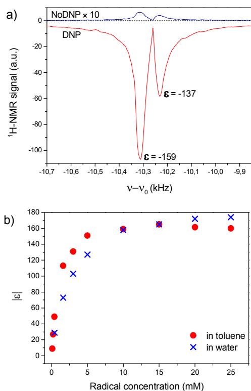
Fig. 1 a) ^1\text{H} NMR spectra of toluene doped with 5 mM TEMPONE-D- ^{15}\text{N} at 14 MHz. b) Concentration dependence of DNP enhancements (from maximum of \epsilon_{\text{FID}} ) of TEMPONE-D- ^{15}\text{N} in toluene and in water. Experimental details for toluene: samples degassed with three freeze-pump-thaw cycles, volumes of 20 \mu\text{L} , 1 or 8 scans for DNP measurement, 128 scans for Boltzmann measurements, P_{\text{mw}} \approx 3 W, t_{\text{irrad.}} = 2 - 30 s depending on concentration. For aqueous samples: non-degassed, V = 0.6 \mu\text{L} , 64 scans for DNP measurements and 1024 scans for Boltzmann measurements, t_{\text{irrad.}} = 1 - 5 s. Details on the experimental set up were given in Ref. 23 and in SI.
