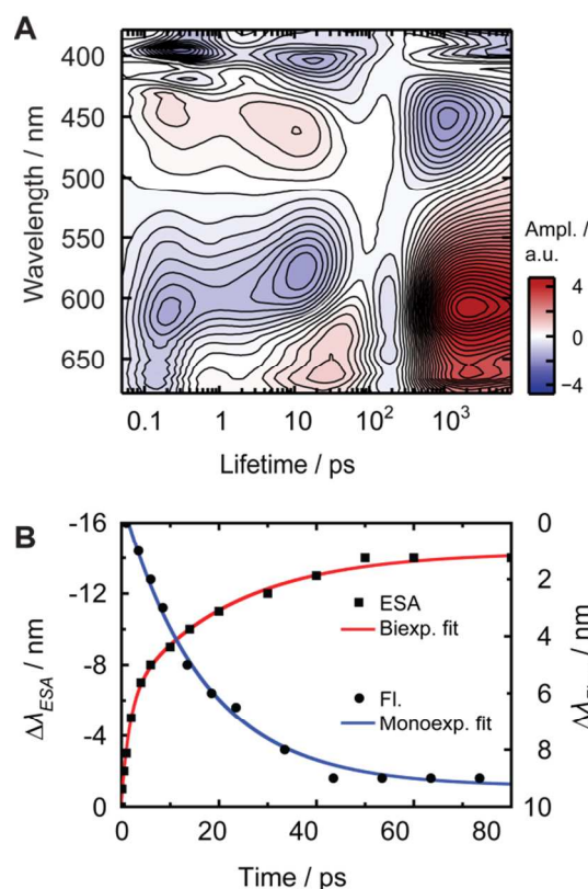
Fig. 4: Analysis of PyA in MeOH and 1% DMSO excited at 388 nm. A: Lifetime density amplitude map. B: Spectral shift of the unstructured ESA2 maximum (cubes) and biexponential fit (red line, \tau_{ESA2^a} = 1.8 \pm 0.3 ps and \tau_{ESA2^b} = 22 \pm 3 ps), as well as spectral shift of the fluorescence maximum (circles) measured with the streak camera and monoexponential fit (blue line, \tau_{SE2b} = 17 \pm 1 ps).
