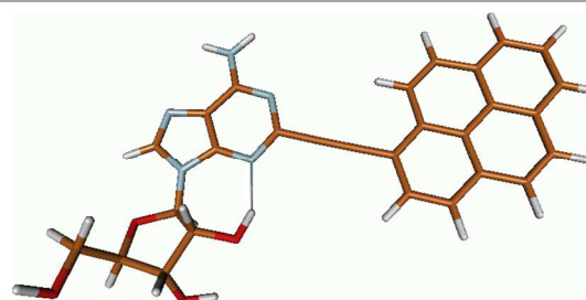
Fig. 6: Ground state optimized structure of PyA (DFT/BH-LYP).
