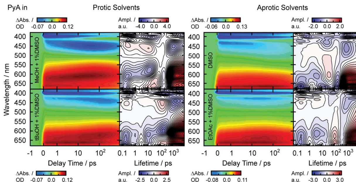
Fig. 5: Transient absorption spectra ( \lambda_{exc} = 388 nm) and LDM of PyA in protic solvents (MeOH and tBuOH, left side) and in aprotic solvents (DMSO and EtOAc, right side). MeOH and DMSO as the upper limit of the measured permittivity range of each solvent class and tBuOH and EtOAc as the lower limit.
