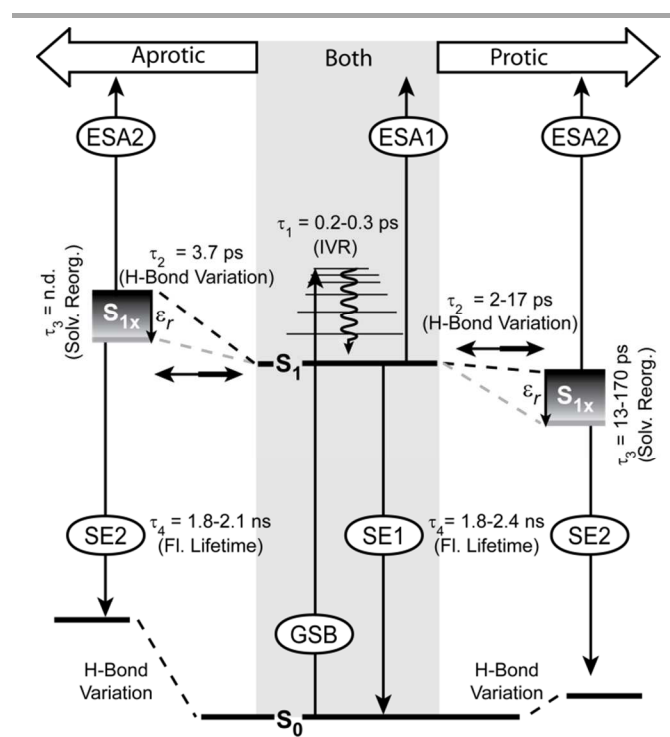
Fig. 7: Modell of relaxation pathways and observed signals in the TA for PyA in aprotic (left side) and protic (right side) solvents.
