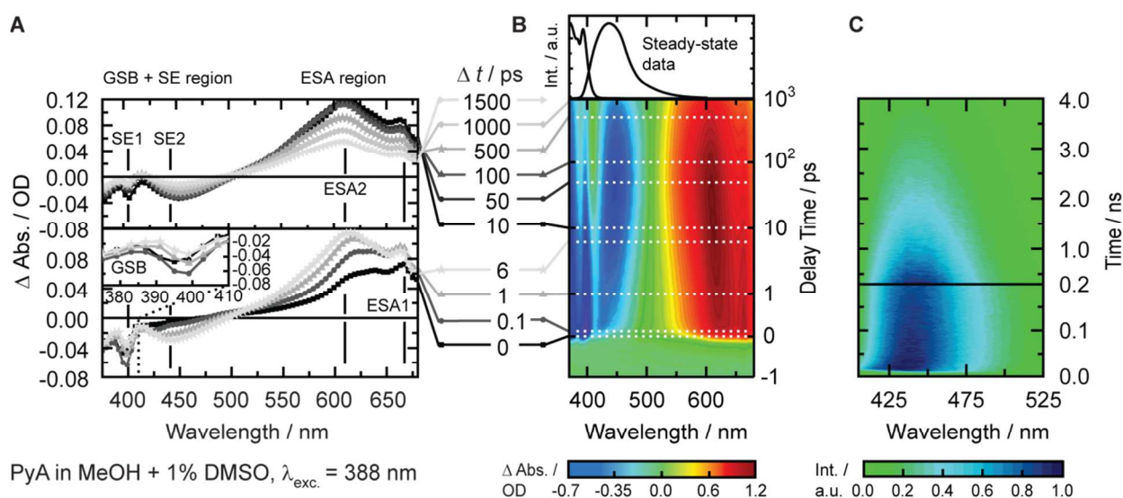
Fig. 3: Dataset for PyA in MeOH and 1% DMSO excited at 388 nm. A: Time slices between 0 ps and 6 ps (lower panel) as well as 10 ps and 1500 ps (upper panel). Inlet shows GSB with superimposed SE. B: Contour plot between -1 ps and 1000 ps, with highlighted positions of time slices (dashed lines). C: Streak camera measurements with a \sim 5 ns decay window (upper panel) and a \sim 0.5 ns decay window (lower panel).
