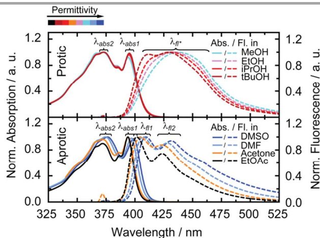
Fig. 2: Normalized absorption (solid lines) and normalized fluorescence (dashed lines) spectra for pyrene modified adenosine (150 \mu\text{M} and 10 \mu\text{M} , respectively) in four protic (upper panel) and four aprotic (lower panel) solvents. For the fluorescence spectra PyA was excited at \lambda_{abs2} : MeOH - 372 nm, EtOH, iPrOH and tBuOH - 373 nm, DMSO - 376 nm, DMF - 374 nm, Acetone and EtOAc - 372 nm.
