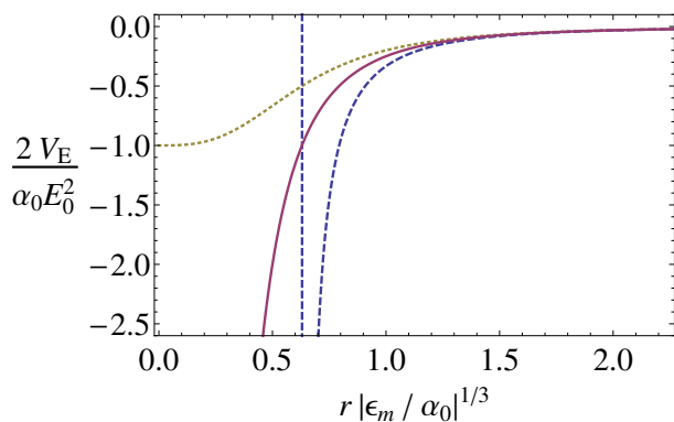
Fig. 3 The interaction energy V_E / (\frac{1}{2}\alpha_0 E_0^2) of a Lorentz atom (LA) with polarizability \alpha_0 with a conducting half-space at zero potential, as a function of the dimensionless distance r |\epsilon_m / \alpha_0|^{1/3} between the LA and the half-space, in the presence of an external electric field of magnitude E_0 and direction normal to the surface of the half-space. Plotted is the case \alpha_0 > 0 (blue dashed line), \alpha_0 < 0 (yellow dotted line), as well as the large-distance approximation (solid line), for which the sign of \alpha_0 is irrelevant. The vertical dashed line at r |\epsilon_m / \alpha_0|^{1/3} \approx 0.63 corresponds to the polarization catastrophe that occurs for positive polarizabilities.
