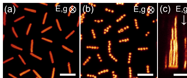
Fig. 7 Rods with length l = 3.3 \mu\text{m} and diameter d = 550 \text{ nm} in an electric field E = 0.5 \text{ V}/\mu\text{m} . The spacing between the electrodes was approximately 15 \mu\text{m} . (a) Rods on the bottom electrode oriented parallel to the electrode surface (flat). The rods still performed (in plane) rotational and translation motion. (b) First layer of rods standing on top of the flat rods. (c) A side-view shows that several layers of rods were positioned on top of the flat ones. The scale bars are 5 \mu\text{m} .
