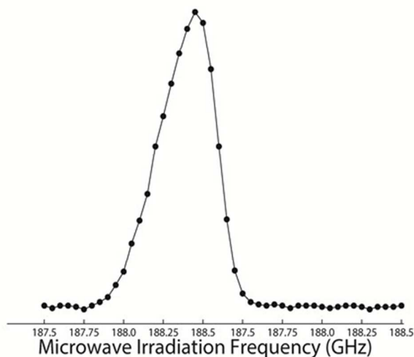
Figure 5. Longitudinally detected electron spin resonance (LODESER) spectrum of a sample of 12 mM DPPH in toluene, taken at 4.2 K. A TEMPOL spectrum obtained with this probe is shown in ref [34].
