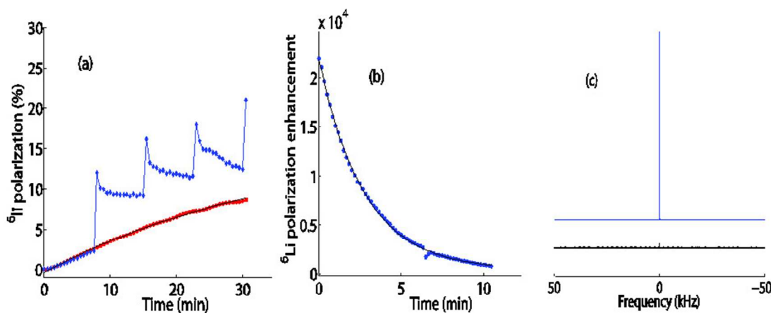
Figure 4. (a) Experimental build-up of P(^6\text{Li}) obtained with cross polarization (blue), with DNP only (red) and fit of the latter curve (black) at 6.7 T and 1.2 K. Since the proton build-up time constant was \tau_{\text{DNP}}(^1\text{H}) = 3.58 min, intervals of 7.5 min between subsequent CP contacts were used as a compromise between the build-up of P(^1\text{H}) and the decay of P(^6\text{Li}) . After each CP contact, the polarization P(^6\text{Li}) tends to return to the plateau observed by direct ^6\text{Li} DNP. (b) Detail of the decay of P(^6\text{Li}) in solution at 7 T and 300 K (blue), fitted to a mono-exponential function (black). The sample consisted of 4 beads of 10 \mu\text{l} each of 7 M ^6\text{Li} -enriched lithium chloride LiCl with 50 mM TEMPO in 40:40:20 (v:v:v) ethanol- \text{d}_6 : \text{D}_2\text{O} : \text{H}_2\text{O} with an extra bead of 10 \mu\text{l} of 3 M ascorbic acid in \text{H}_2\text{O} to quench the radicals during dissolution. (c) Detail of two ^6\text{Li} spectra taken at room temperature with a single flip angle of 5^\circ (blue) and gain 16 and a single 90^\circ flip angle and gain 1024. Spectra are scaled to fit in the graph.
