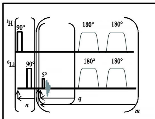
Figure 1. Pulse sequence used for cross-polarization (CP) in solids at low temperatures [5-7]. Both protons and ^6\text{Li} nuclei are initially saturated by a series of 90^\circ pulses (typically n = 20 ) spaced by 10 ms. Two nested loops ( q inside m ) are used, the inner loop to measure the polarization of ^6\text{Li} with small 5^\circ flip angles, and the outer loop (typically m = 18 with intervals of 10 s for samples at 4.2 K or 30 s at 1.2 K) to establish cross polarization contacts by simultaneously applying pairs of frequency-modulated inversion pulses. The EPR transitions are saturated throughout the experiment to induce DNP.
