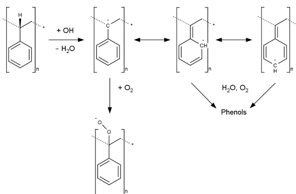
Scheme 3: Proposed mechanism for generation of redox-active phenolic groups on the PS surface through reaction with hydroxyl radicals.
