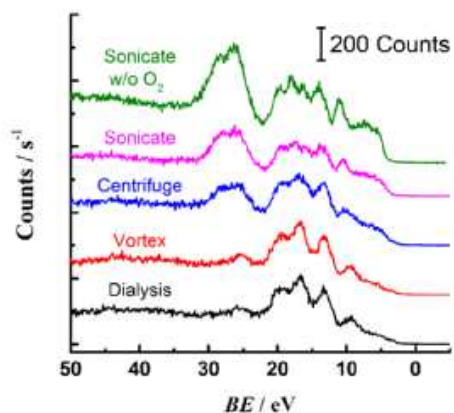
Figure 4: Valence band XPS spectra for polystyrene cleaned by dialysis (black); cleaned by centrifugation (blue); subject to 1 hour sonication in air-saturated solution (pink); subject to 1 hour sonication in deoxygenated solution (green) and subject to 1 hour vortex mixing (red).
