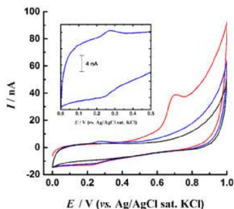
Figure 1: CV in 0.2 M pH 6 PBS of centrifuged PS immobilised on BDD electrode. Red: 1 st scan; Blue: 2 nd scan; Black: background response of unmodified BDD. Scan rate 0.02 \text{V s}^{-1} .
