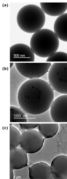
Figure 5: TEM images of (a) dialysed PS; (b) PS sonicated for 1 hour; (c) PS vortexed for 1 hour.
