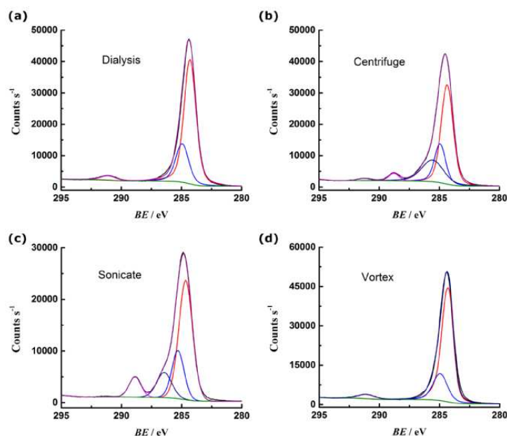
Figure 3: Carbon 1s region XPS spectra for PS (a) cleaned by dialysis; (b) cleaned by centrifugation; (c) subject to 1 hour sonication; (d) subject to 1 hour vortex mixing.
