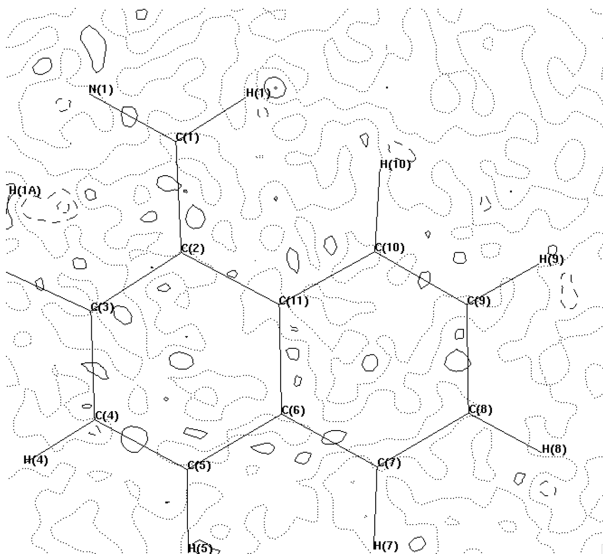
Figure 2 Residual density from multipole model in the plane of C(1), N(1) and C(2), displayed at the 0.1 \text{ e} \cdot \text{\AA}^{-3} contour level.
