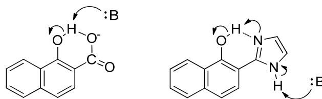
Scheme 5. Deprotonation reaction paths for 1-hydroxy-2-naphthoate and the HA species of 2NI1OH.
