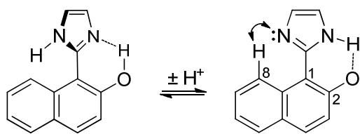
Scheme 4. IMHB interactions on 1NI2OH n and 1NI2OH - species.
