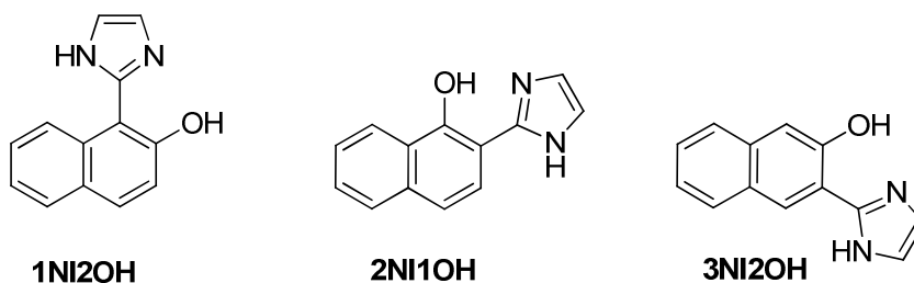
Scheme 1. Constitutional isomers of ortho -(1 H -imidazol-2-yl)naphthol studied in this work.
