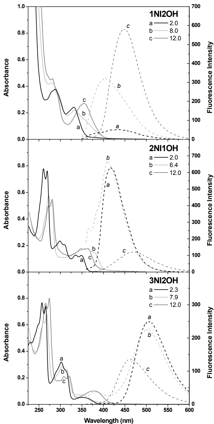
Figure 1. Absorption (solid line) and emission (broken line) spectra for 1-(1 H -imidazol-2-yl)naphthalen-2-ol (1NI2OH, 5.96 \times 10^{-5} M), 2-(1 H -imidazol-2-yl)naphthalen-1-ol (2NI1OH, 2 \times 10^{-5} M) and 3-(1 H -imidazol-2-yl)naphthalen-2-ol (3NI2OH, 2 \times 10^{-5} M) in water at the different indicated pHs and 25 °C. The excitation wavelength for 1NI2OH was 330 nm and for 2NI1OH and 3NI2OH were 350 nm.
