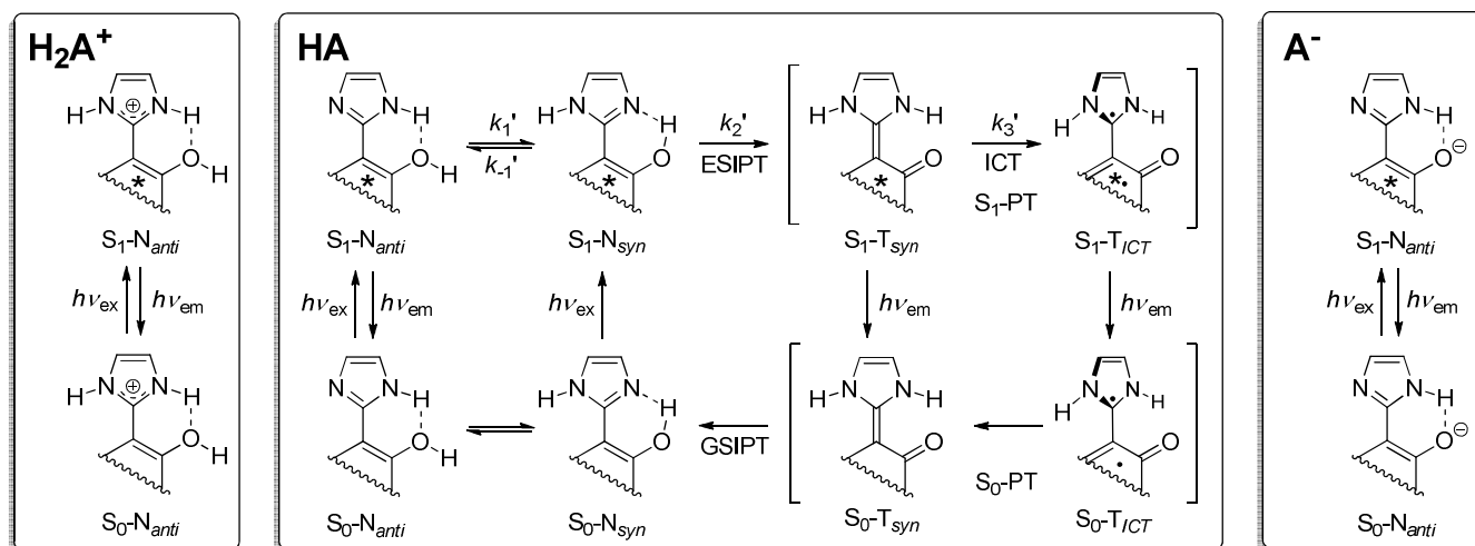
Scheme 3. Structures of various ground and excited state acid-base species for ortho -(1 H -imidazol-2-yl)naphthol constitutional isomers. H_2A^+ , HA and A^- respectively are the cationic, neutral and anionic species.
