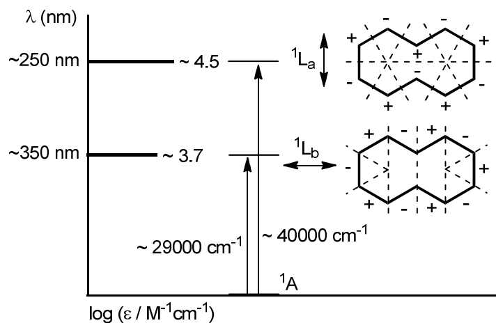
Figure 2. Electronic energy levels of naphthalene and polarization diagrams for low absorption bands. Energies and \log \epsilon are average of measurements for the neutral species of ortho -(1 H -imidazol-2-yl)naphthols.
