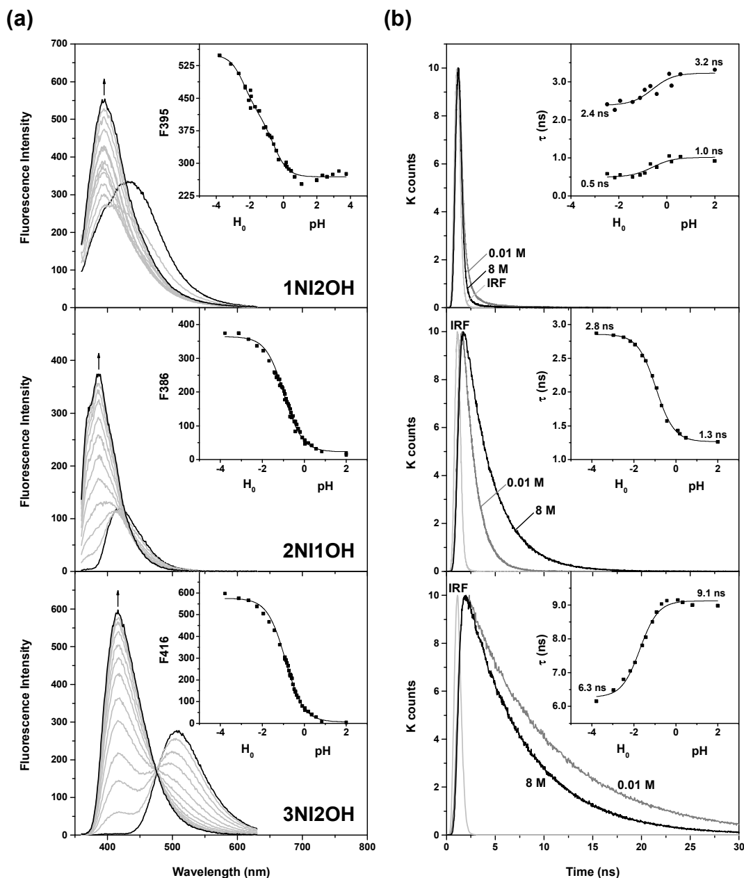
Figure 3. Fluorimetric titrations in water from [HCl] 0.01 to 8 M at 25 °C for 1-(1 H -imidazol-2-yl)naphthalen-2-ol (1NI2OH, 3 \times 10^{-5} M), 2-(1 H -imidazol-2-yl)naphthalen-1-ol (2NI1OH, 3 \times 10^{-5} M) and 3-(1 H -imidazol-2-yl)naphthalen-2-ol (3NI2OH, 2 \times 10^{-5} M): (a) Emission spectra at \lambda_{\text{ex}} of 330 nm for 1NI2OH and 350 nm for 2NI1OH and 3NI2OH. Inserts show the pH/ H_0 -dependence of the fluorescence intensities (F) at the wavelengths indicated by arrows. The solid lines are fits according to Eq. 2; (b) Fluorescence decays and instrumental response functions (IRF) profiles for representative measurements at \lambda_{\text{ex}} of 330 nm using the respective \lambda_{\text{em}} of 450, 400 and 462 nm for 1NI2OH, 2NI1OH and 3NI2OH. The inserts show pH/ H_0 -dependence of the lifetime. The solid lines were obtained from nonlinear least-square fit using the Eq. 1 and the limiting \tau values shown in the graphs. The value at pH 2 for 1NI2OH was taken as the average of measurements at pH 2.0, 4.0 and 8.0.
