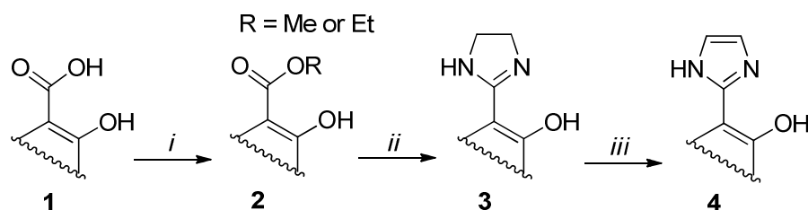
Scheme 6. Synthetic route for preparation of the ortho -(1 H -imidazol-2-yl)naphthols 4 : Conditions: i . RI, \text{KHCO}_3 , solv. DMF; ii . Ethylenediamine, reflux; iii . Pd/C 10%, solv. \text{Ph}_2\text{O} .
