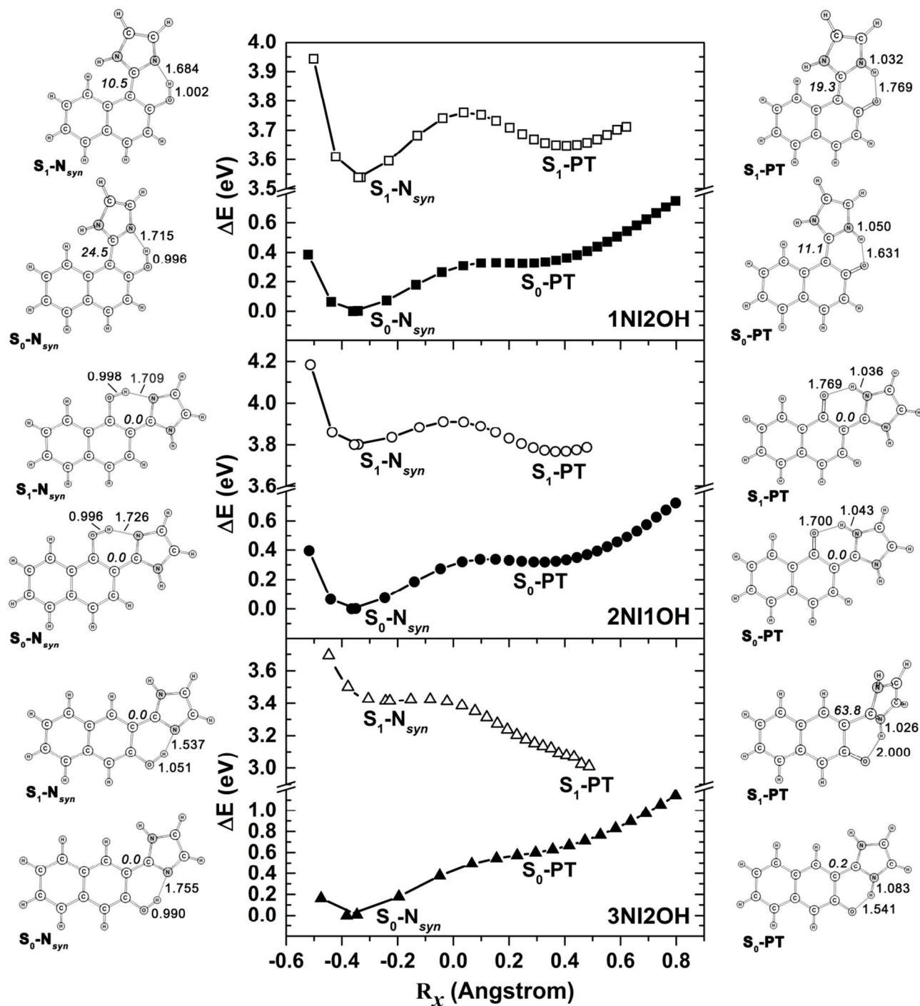
Figure 4. Potential energy surface for the proton transfer in the ground state ( S_0 ) and first ( S_1 ) \pi,\pi^* excited state of 1NI2OH, 2NI1OH and 3NI2OH, and the corresponding structures for the N_{syn} and the PT forms of either S_0 or S_1 states. The bond lengths for O-H (in N_{syn} ), N-H (in PT) and IMHB are shown in angstroms, while the torsional angle for the interannular bond between the naphthol and the imidazole ring are shown in italic and degrees.
