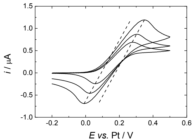
Fig 7. Cyclic voltammograms in 0.638\text{ mM} DMFc in supercritical \text{CO}_2 with 15\text{ wt}\% MeCN containing 20\text{ mM } [\text{NBu}^n_4][\text{BF}_4] supporting electrolyte. T = 309\text{ K} . p = 17.51\text{ MPa} . The working electrodes was a 0.5\text{ mm} diameter platinum gold disc, the counter and reference electrode were 0.5\text{ mm} diameter platinum wires. Sweep rate 100, 200 and 500\text{ mV/s} .
