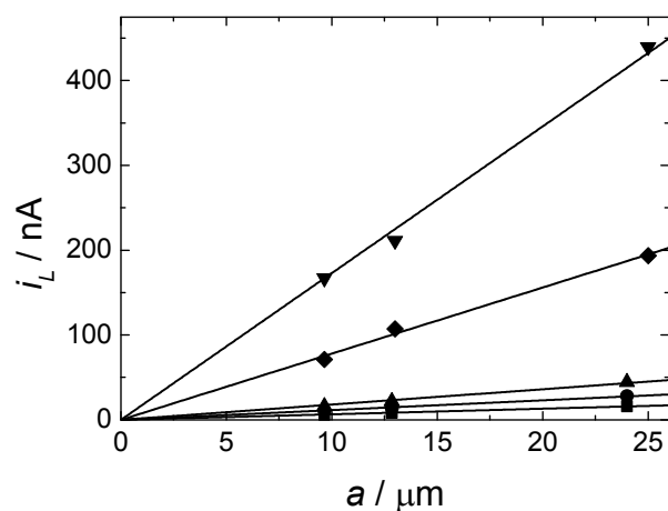
Fig. 6. Plot of diffusion limited current versus the electrode radii for a series of cyclic voltammograms in supercritical CO 2 with 15 wt% MeCN and 20 mM [NBu n ] 4 [BF 4 ] electrolyte. T = 309 K. p = 17.24 - 17.72 MPa. The concentrations were 0.43 (■), 0.78 (●), 1.07 (▲), 5.20 (◆), and 11.0 mM (▼). The counter and reference electrode were 0.5 mm diameter platinum wires.
