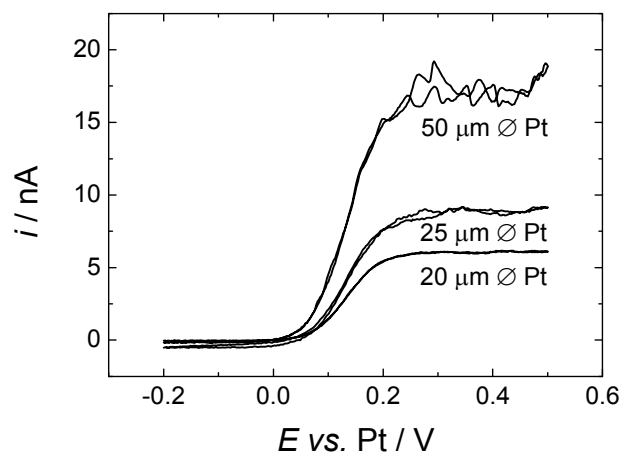
Fig. 2. Cyclic voltammetry of 0.43 mM DMFc in supercritical CO 2 with 15 wt% MeCN containing 20 mM [NBu 4 ][BF 4 ] supporting electrolyte at 309 K. The working electrodes were a 20, 25 and 50 μm diameter platinum disc, the counter and reference electrode were 0.5 mm diameter platinum wires. p = 17.51 MPa, p = 17.55 MPa, p = 17.60 MPa respectively. Sweep rate 10 mV s -1 for all electrodes.
