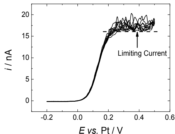
Fig. 3 Cyclic voltammograms in 0.43 mM DMFc in supercritical CO 2 with 15 wt% MeCN containing 20 mM [NBu 4 ][BF 4 ] supporting electrolyte. T = 309 K. p = 17.60 MPa. The working electrode was a 50 \mu\text{m} diameter platinum disc, the counter and reference electrode were 0.5 mm diameter platinum wires. Sweep rate 10 \text{mV s}^{-1} .
