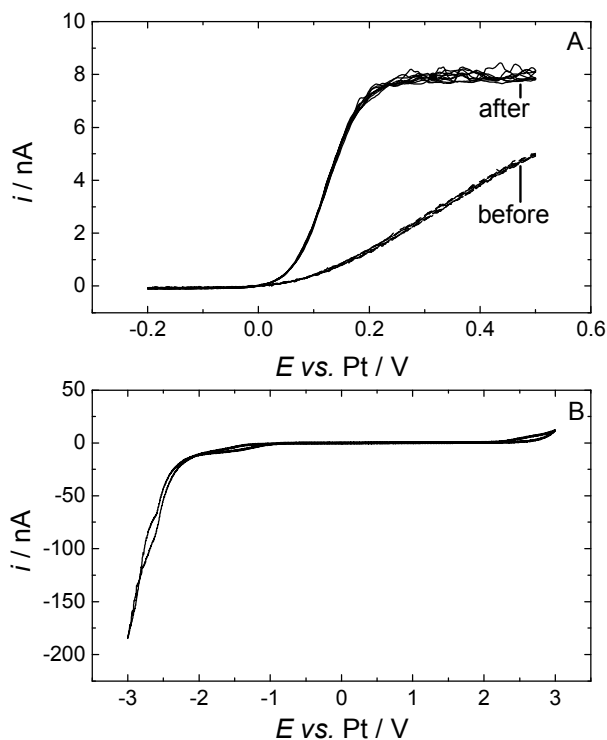
Fig. 1. Cyclic voltammetry of 0.43 mM DMFc in supercritical CO 2 with 15 wt% MeCN containing 20 mM [NBu 4 ][BF 4 ] supporting electrolyte at 309 K. The working electrode was a 25 μm diameter platinum disc, the counter and reference electrode were 0.5 mm diameter platinum wires. p_A = 17.50 MPa, p_B = 17.43 MPa. Voltammograms for figure A were recorded at 10 mV s -1 , figure B at 100 mV s -1 .
