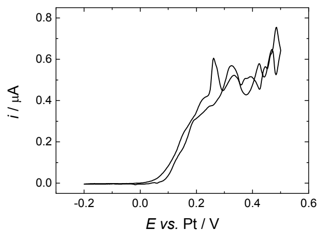
Fig 8. Cyclic voltammetry in 0.638\text{ mM} DMFc in supercritical \text{CO}_2 with 15\text{ wt}\% MeCN containing 20\text{ mM } [\text{NBu}^n_4][\text{BF}_4] supporting electrolyte. T = 309\text{ K} . p = 17.51\text{ MPa} . The working electrodes was a 0.5\text{ mm} diameter platinum gold disc, the counter and reference electrode were 0.5\text{ mm} diameter platinum wires. Sweep rate 10\text{ mV/s} .
