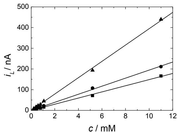
Fig. 5. Plot of diffusion limited current versus the decamethylferrocene concentration for a series of cyclic voltammograms in supercritical CO 2 with 15 wt% MeCN and 20 mM [NBu n ] 4 [BF 4 ] electrolyte. T = 309 K. p = 17.24 - 17.72 MPa. The working electrodes were a 20 (■), 25 (●) and 50 μm (▲) diameter platinum disc, the counter and reference electrode were 0.5 mm diameter platinum wires.
