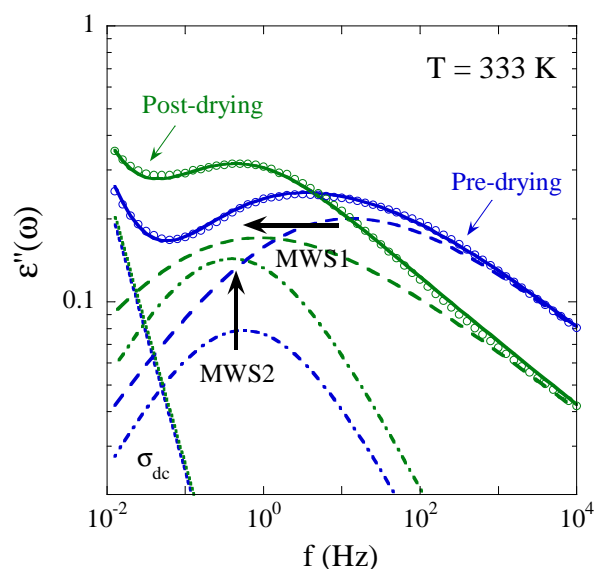
Fig. 3 Imaginary permittivity data at 333 K for a ( \Phi_{\text{si}} = 8.4\%v , 50%D3)-nanocomposite before and after drying. Solid lines are fits to the experimental data by means of eq 1. The relaxation time of the individual contribution MWS1 (dashed lines) is seen to be sensitive to drying, whereas MWS2 (dashed-dotted lines) remains at the same position. Pre- and post-drying ionic conductivity are shown as superimposed dotted lines.
