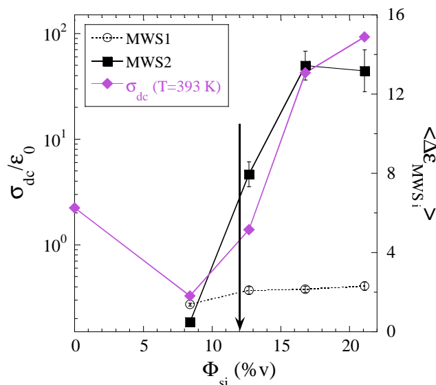
Fig. 6 DC-conductivity at 393 K (diamonds) and average value of the dielectric strengths over T for MWS1 (circles) and MWS2 (squares) as a function of filler fraction (50%D3). Lines are guide for the eyes. The percolation threshold as obtained from rheology 6 is indicated by an arrow.
