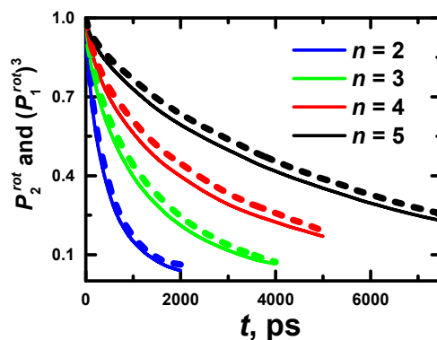
Figure B.2. The time dependencies of P_2^{rot} and (P_1^{rot})^3 for PLL dendrimers with n = 2-5 at 300 K.
