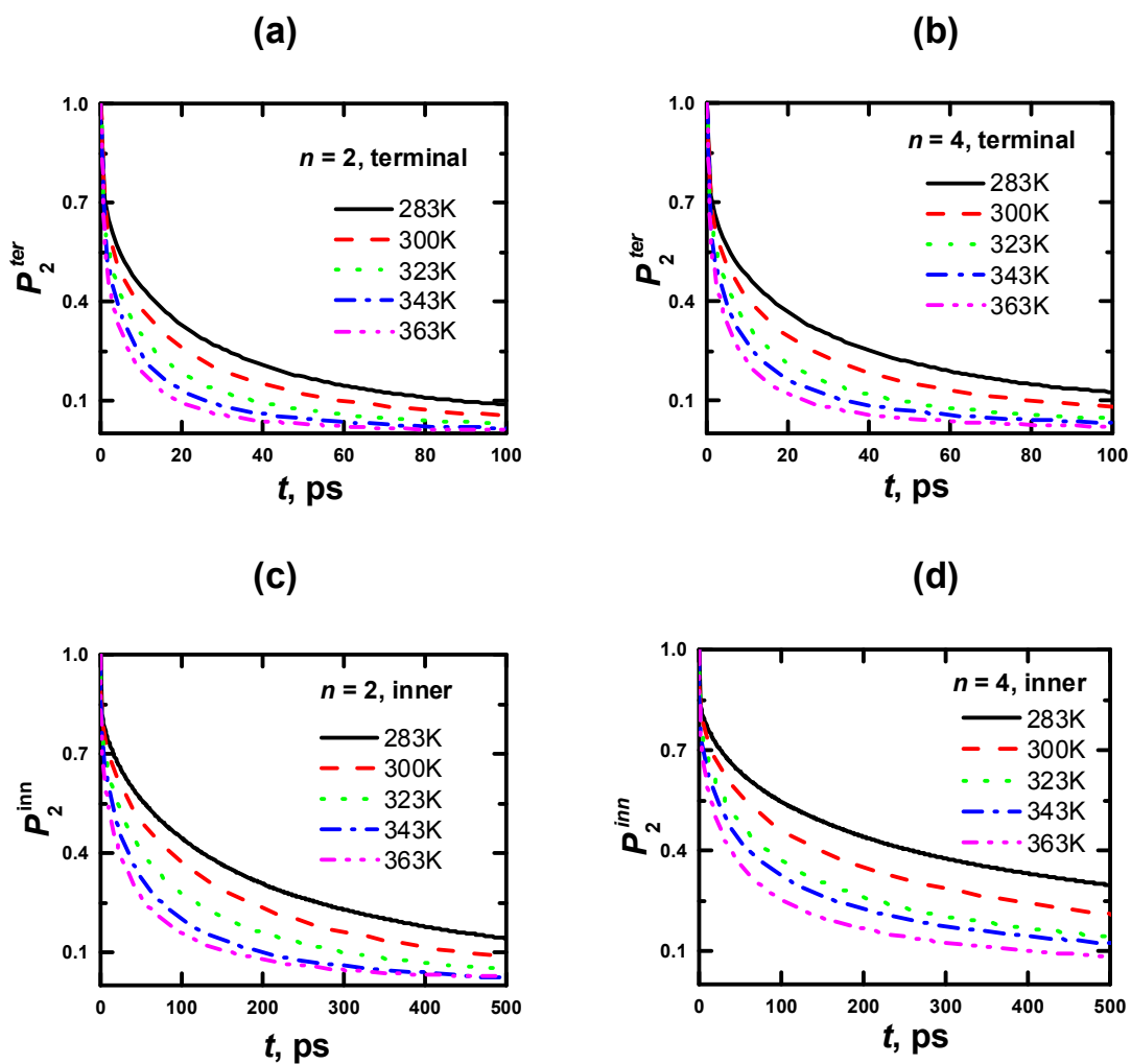
Figure A.2. Time dependences of P_2 ACF for the r_{HH} vectors of CH_2 groups of the PLL dendrimer terminal (a, b) and inner (c, d) segments with n = 2 (a, c) and 4 (b, d) at different temperatures.
