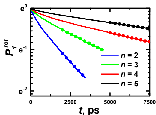
Figure B.1. The time dependencies of P_1^{rot} ACF for PLL dendrimers with n = 2-5 at 300 K. Dotted lines are the approximation of the \ln(P_1^{rot}) slope.
