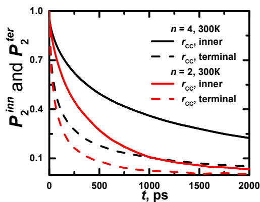
Figure A.3. Time dependences of P_2 ACF for the r_{CC} vectors in inner and terminal segments of PLL dendrimers with n = 2 and 4 at 300 K.
