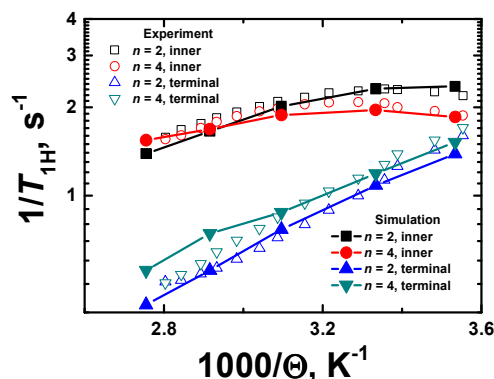
Figure 7. Plots of 1/T_{1H} vs. vs. inverse temperature ( 1000/\Theta ) for terminal and inner CH_2 groups. The NMR experimental data 40 and the MD simulation results are shown.
