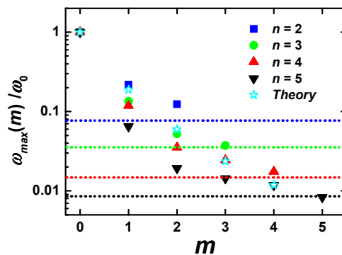
Figure 4. The position of the [1/T_{1H}] maxima for different m and n . Dotted horizontal lines mark \omega_{rot} and correspond to n with the same color; \omega_0 = \omega_{max}(m=0) . MD simulation and analytical theory 47 results.
