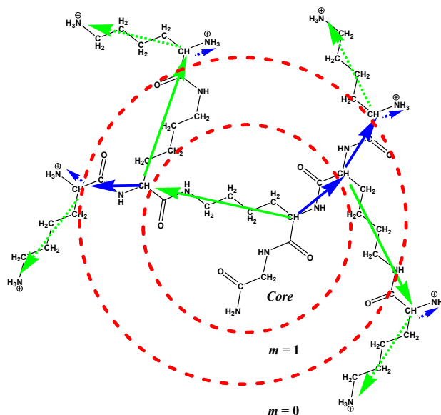
Figure 1 The chemical structure of the n = 1 generations PLL dendrimer. The solid blue and green arrows are the vectors connecting C atoms of branching points for short and long inner segments, respectively. The dotted arrows are the vectors connecting C atoms of terminal branching points and N atoms of terminal \text{NH}_3 groups. m is the dendrimer layer number.
