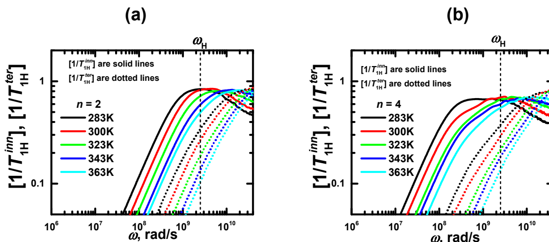
Figure 5. Frequency dependences of [1/T_{1H}] for \text{CH}_2 groups of inner and terminal segments of lysine dendrimers with n = 2 and 4. The vertical dotted line indicates the frequency ( \omega_H/2\pi = 400 MHz) corresponding to the spectrometer used in Ref. 40 .
