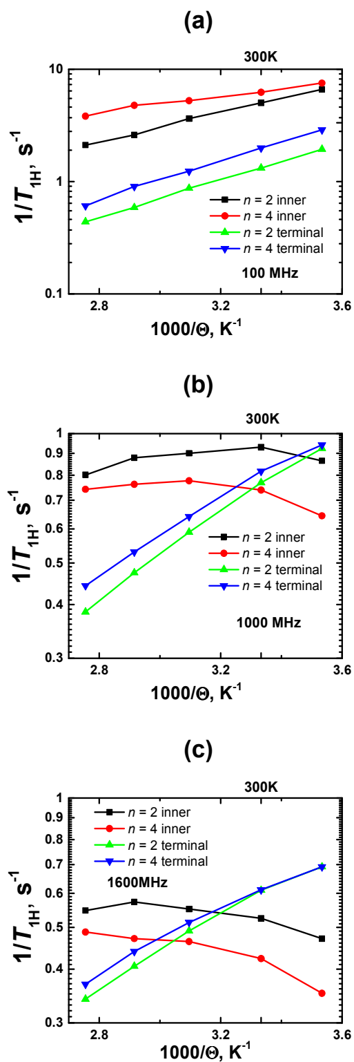
Figure 8. Plots of 1/T_{1H} vs. inverse temperature ( 1000/\Theta ) for terminal and inner \text{CH}_2 groups at different \omega_H/2\pi = 100, 1000 and 1600 MHz. MD simulation results.
