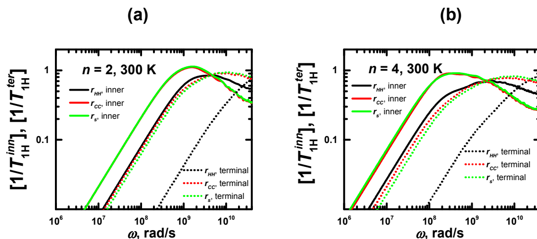
Figure 6. Frequency dependences of 1/T_{1H} for r_{HH} , r_{CC} , and r_s , calculated for inner and terminal segments of lysine dendrimers with n = 2 u 4 at 300 K
