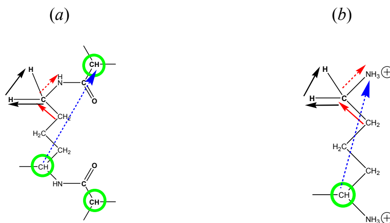
Figure 2. Chemical structure of an internal segment (a) and a terminal segment (b). The green circles mark branching points. The black arrows correspond to the direction of \mathbf{r}_{HH} and \mathbf{r}_{CH} unit vectors of CH_2 groups, which are observed in the NMR relaxation. The red arrows are \mathbf{r}_{CC} and \mathbf{r}_{CN} vectors of CC and CN bonds, which are connected in the CH_2 group, and the dotted blue arrows mark the long segment vector, \mathbf{r}_s . The orthogonal vector is determined
