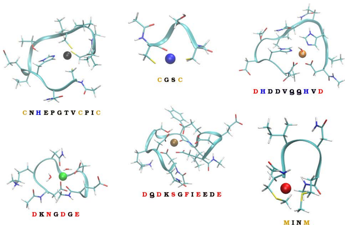
Figure 1: The six studied peptides. The peptides are abbreviated by the amino-acid residues participating in binding of a metal ion. The larger peptides ( CHCC , DHHD , DNDO , DDSOEE ) are based on structures found in MESPEUS database. 38 The smaller two peptides ( CC , MM ) come from previous research in our laboratory. 39 Vid Section 2.2 for details.
