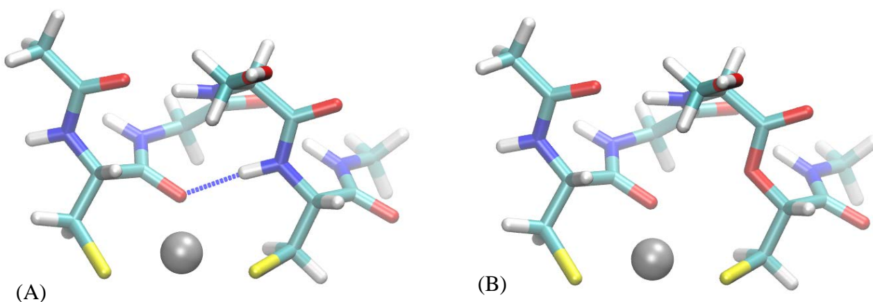
Figure 3: Esther analogues of peptides. An example of substitution of N-H hydrogen bond donor (A) with O (B) in CC peptide. The substitution does not perturb geometry, but does eliminate the hydrogen bond.
