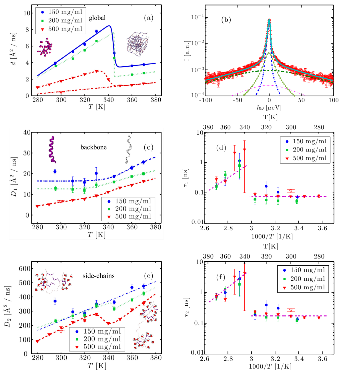
Fig. 3 (a) Apparent self-diffusion coefficient d as a function of T for c_p = 150, 200 and 500 mg/ml (symbols) and fits with equation (7) (lines). The illustrations depict a colloidal suspension of native proteins (left) and a cross-linked network of denatured proteins (right). (b) Example spectrum (symbols) of aqueous BSA at c_p = 500 mg/ml, T = 370 K and q = 0.45 \text{ \AA}^{-1} . The solid line superimposed on the data is a fit of the model function (equation (6)). The blue dot-dashed line depicts the Lorentzian describing the protein global self-diffusion, while the light green asterisks and the dark green dashed line represent the Lorentzians attributed to backbone and side-chain dynamics, respectively. The magenta dots denote the contribution of D 2 O. (c) D_1 as a function of T (symbols). D_1 is attributed to the dynamics of the backbone and sensitive to the secondary structure, part of which undergoes a transition from \alpha -helix (left image) to disordered coil (right image). The illustration of a helix-to-coil transition was rendered with VMD 71 . The lines are guides to the eye. (d) Arrhenius plot of the residence time \tau_1 between two jumps of the side-chains versus T for three c_p (symbols). The data above denaturation were fitted with an Arrhenius equation (line), while at low temperatures the line is a guide to the eye. (e) D_2 as a function of T for the concentrations reported in the legend (symbols). D_2 is associated with the dynamics of the side-chains. The lines are guides to the eye. The illustrations depict solvent-inaccessible side-chains in the folded protein (left) becoming solvent-exposed in the unfolded protein (right). (f) Arrhenius plot of the residence time \tau_2 as a function of T (symbols). \tau_2 is the time a side-chain needs to switch between two conformations during which they are considered immobile with respect to the backbone. The data above denaturation were fitted with an Arrhenius equation (line). The red open triangles in (a), (c)-(f) refer to the sample at 500 mg/ml cooled back to room temperature after denaturation.
