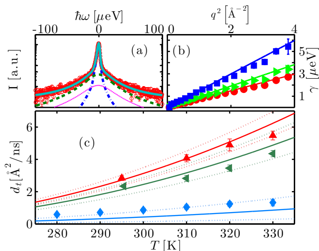
Fig. 2 (a) Example spectrum (symbols) recorded using the neutron backscattering spectrometer BASIS, SNS, ORNL, on bovine serum albumin (BSA) at the concentration c_p = 200 mg/ml in heavy water ( \text{D}_2\text{O} ) at the temperature T = 295 K. The displayed data have been detected at the scattering vector q = 0.45 \text{ \AA}^{-1} . The solid line superimposed on the data is a fit of the model function (equation 1) containing two Lorentzians accounting for the dynamics of the protein molecules (blue and green dashed lines) and a fixed contribution accounting for \text{D}_2\text{O} (magenta dotted line), convoluted with the resolution function. (b) Linewidth \gamma of the Lorentzian accounting for the translational and rotational diffusion of the entire protein as a function of q^2 for c_p = 500 mg/ml at T = 280, 290 and 310 K (red circles, green triangles and blue squares, respectively). The lines are the fits following the Fickian law \gamma = dq^2 . (c) Translational self-diffusion coefficients d_t as a function of temperature for c_p = 150 mg/ml (red pointing-up triangles), 200 mg/ml (green triangles), and 500 mg/ml (blue diamonds). The solid lines are the respective theoretical self-diffusion coefficients and the dotted lines indicate the confidence interval defined by a relative error of 5% on the ratio between hydrodynamic radius R_h and effective radius R .
