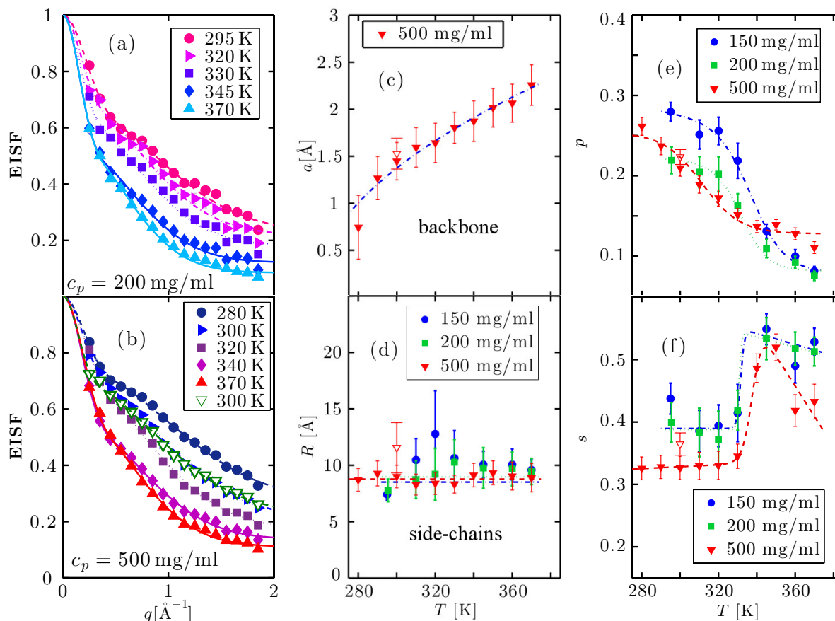
Fig. 4 (a) and (b): EISF as a function of q at the temperatures given in the legend for c_p = 200 and 500 mg/ml, respectively, (symbols) and fits following equation (8) (solid lines). (c) radius a (equation (11)) as a function of T for c_p = 500 mg/ml (symbols) and fit with equation (12) (blue solid line). a is associated with the effective sphere accessible by backbone atoms. (d) Radius R (equation (10)) as a function of T (symbols). The lines are guides to the eye. This radius defines the sphere accessible by side-chain motions. (e) Fraction of immobile atoms p as a function of T (symbols). The lines are guides to the eye. (f) s as a function of T (symbols) defining the ratio of side-chains describable with a diffusion in a sphere model to the total amount of mobile side-chains. The line is a guide to the eye. The parameters in Figures 4(c)-(f) are obtained from the fit of the EISF with equation (8), and the open symbols in Figures 4(b)-(f) refer to the sample at c_p = 500 mg/ml cooled down to room temperature after irreversible denaturation.
