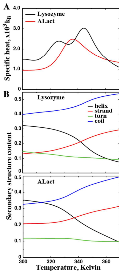
Figure 5. The folding thermodynamics of lysozyme and ALact derived from DMD simulations. (A) The specific heat as a function of temperature. (B) The secondary structure content of alpha helices, beta strands, turns and coils as functions of temperature.
