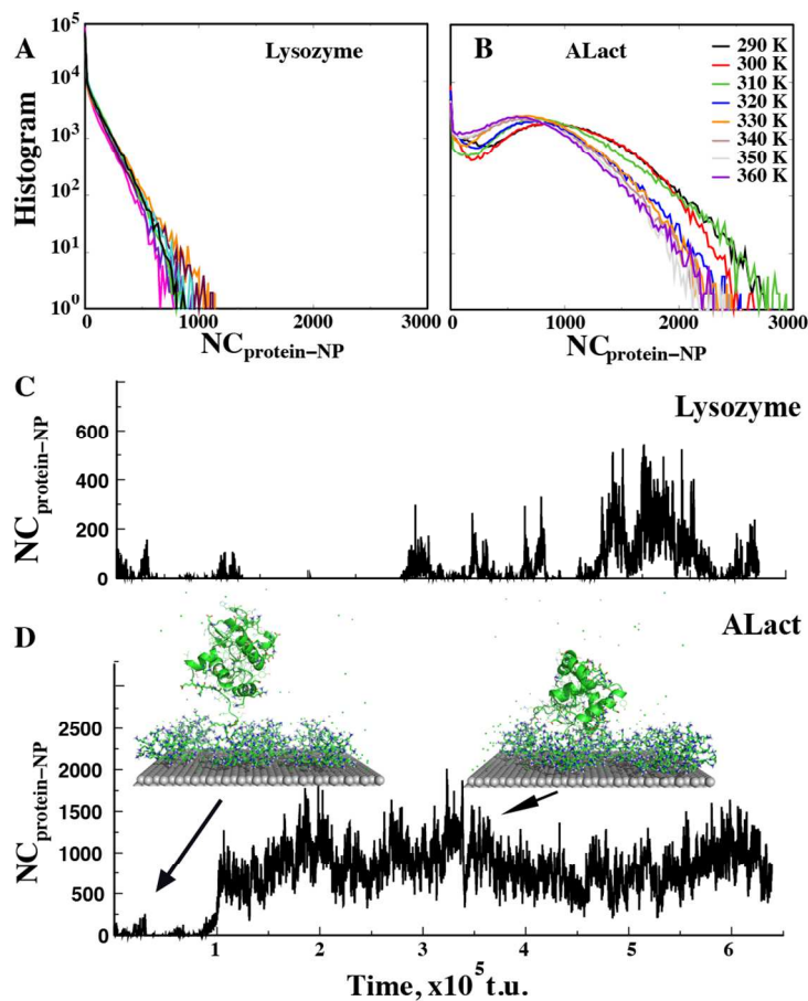
Figure 6. The binding between a bAgNP and lysozyme (A, C) and ALact (B, D). The histogram of intermolecular atomic contacts between protein and NP, NC_{\text{protein-NP}} for lysozyme (A) and ALact (B) are derived from DMD simulations. Results from different temperatures are included. (C) A representative trajectory of lysozyme and bAgNP binding at T = 300\text{K} indicates that the binding is transient and weak. (D) A trajectory of intermolecular contacts between ALact and bAgNP at T = 300\text{K} demonstrates both the weak and strong binding modes. The strong binding with an extensive number of inter-molecular contacts is long lasting.
