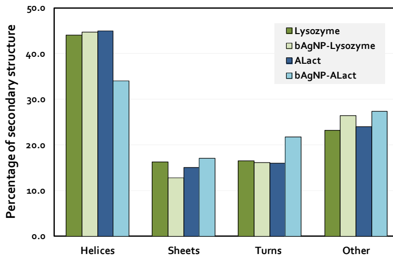
Figure 4. Changes in the secondary structures of lysozyme and ALact upon binding with bAgNPs. The proteins (10 \mu\text{g}/\text{mL} or 0.7 \mu\text{M} in PBS) were pre-incubated with the bAgNPs (2 \mu\text{g}/\text{mL} in PBS) for 2 h at room temperature. The percentages of the secondary structures were calculated by the CDSSTR and CONTIN/LL algorithms of the CDPro package, using SMP56 and SP43 protein reference datasets.
