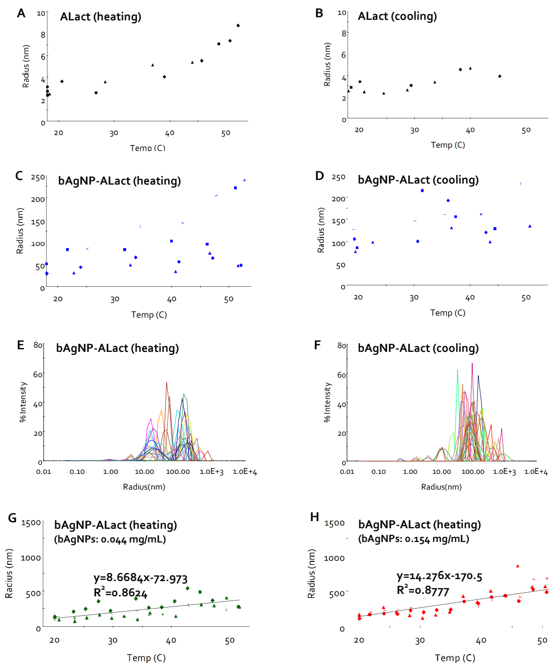
Figure 3. DLS measurement of bAgNP-ALact heated to 53.4°C and cooled back to room temperature. (A, B) Hydrodynamic radius of ALact during heating and cooling. (C, D) Hydrodynamic radius of bAgNP-ALact during heating and cooling. (E, F) Histograms of bAgNP-ALact hydrodynamic radius during heating and cooling. (G, H) Hydrodynamic radius of bAgNP-ALact during heating for different NP:protein ratios. The slopes of the fitted linear trendlines are 8.7 and 14.3 nm/°C, respectively. ALact: 0.9 mg/mL (A-H). bAgNPs: 0.088 (B-F), 0.044 (G) and 0.154 mg/mL (H). All samples in PBS. The diamond, triangles, squares and stars represent data points obtained from different sample wells.
