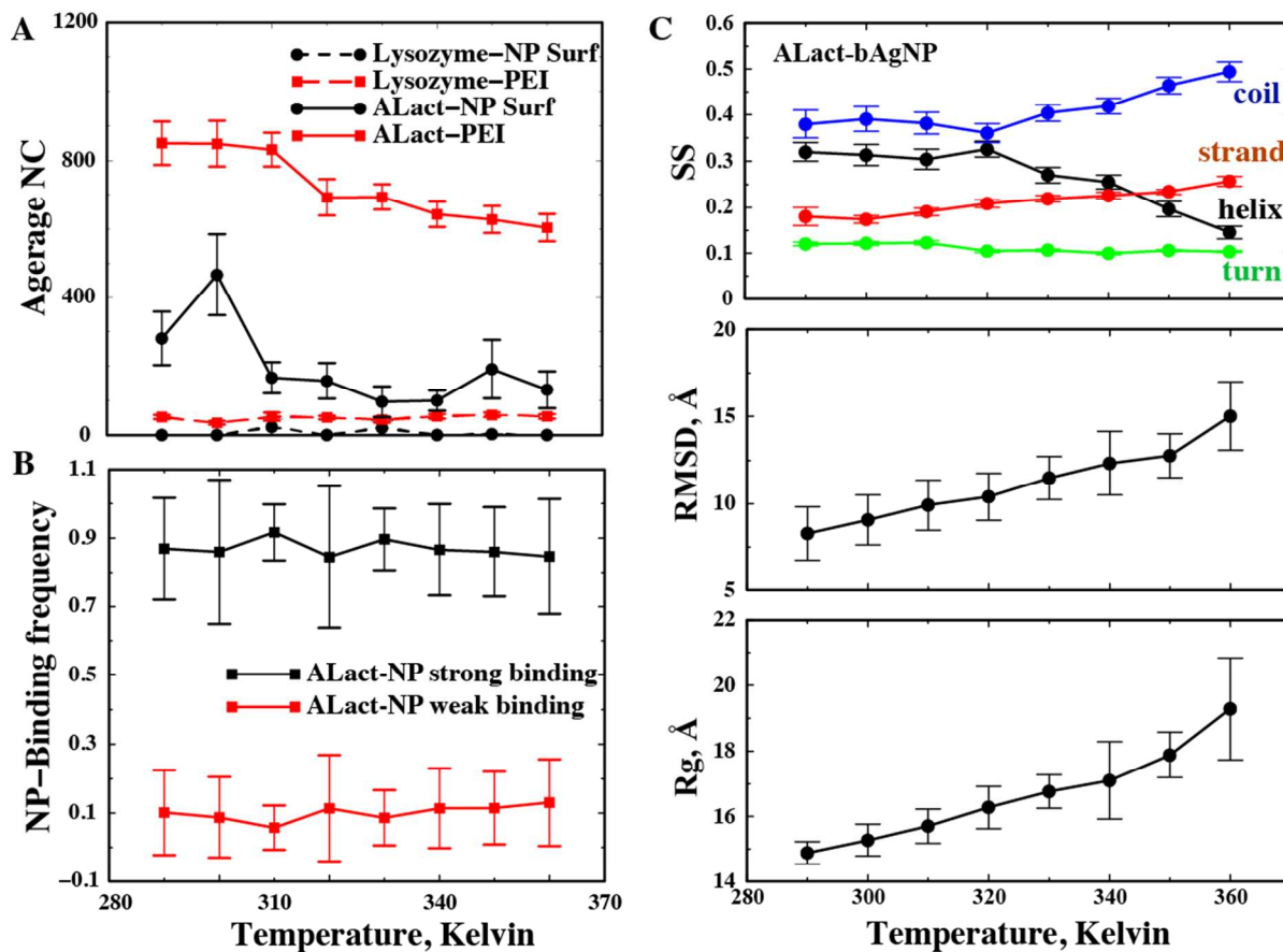
Figure 7. The thermodynamics of bAgNP binding with proteins. (A) The binding of the proteins with the AgNP surface and with PEI was calculated separately as the function of temperature. (B) The frequency of binding between ALact and bAgNP was computed as the function of temperature. The weak and strong binding was identified separately. (C) The structural properties of ALact bound to bAgNP, including secondary structure contents (SS), root-mean-square deviation (RMSD), and Rg, were computed as the function of temperature. The error bars correspond to standard deviations computed from independent simulations at each temperature.
