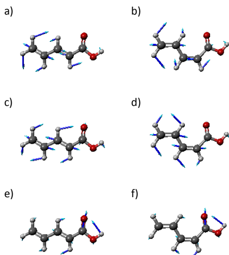
Figure 3. Normal modes of the trans and cis PDA. a) \nu^{\text{a}}_{\text{C}=\text{C}} for the trans isomer, b) \nu^{\text{a}}_{\text{C}=\text{C}} for the cis isomer, c) \nu^{\text{s}}_{\text{C}=\text{C}} for the trans isomer, d) \nu^{\text{s}}_{\text{C}=\text{C}} for the cis isomer, e) \nu_{\text{C}=\text{O}} for the trans isomer, f) \nu_{\text{C}=\text{O}} for the cis isomer.
