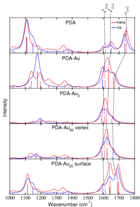
Figure 4. IR spectra of trans (red) and cis (blue) isomers of the different systems as indicated. The line spectra were convoluted by 5 Lorentzians of 20\text{ cm}^{-1} FWHM.
