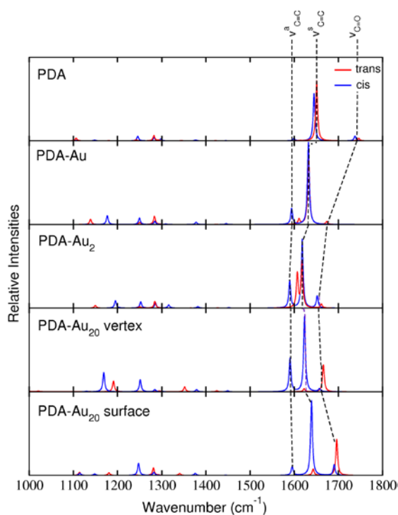
Figure 7. RRS spectra of trans (red) and cis (blue) isomers of the various systems. The line spectra were convoluted by Lorentzians of 5 cm -1 FWHM.
