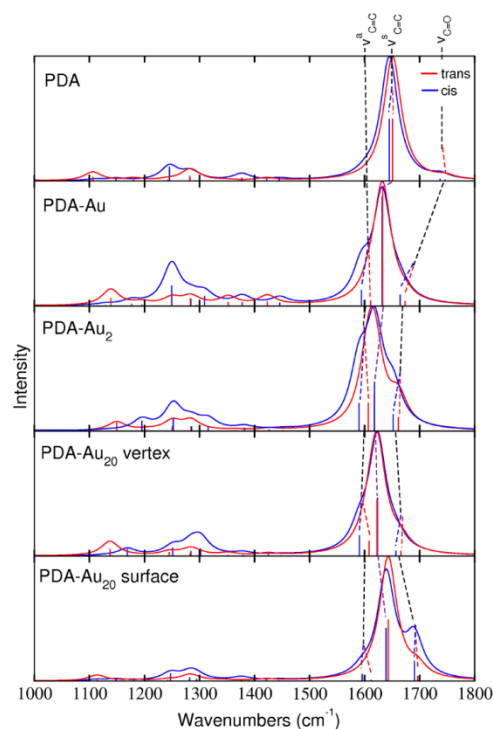
Figure 5. RS spectra of trans (red) and cis (blue) isomers of the different systems as indicated assuming an excitation wavelength of 1064\text{ nm} . The line spectra were convoluted by Lorentzians of 20\text{ cm}^{-1} FWHM.
