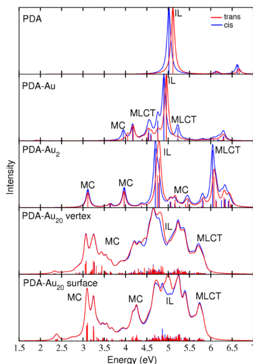
Figure 6. Absorption spectra of trans (red) and cis (blue) isomers for the systems under study. The transitions were broadened by Lorentzians of 0.05 eV FWHM.
