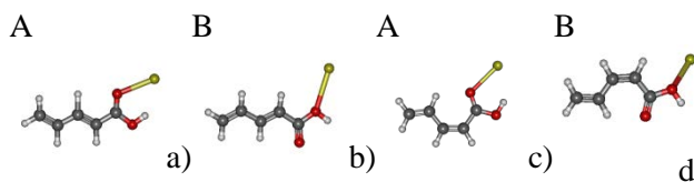
Figure 2. The obtained stable positions for both isomers with 1 Au. a) Position A for the trans isomer, b) Position B for the trans isomer, c) Position A for the cis isomer, d) Position B for the cis isomer.
