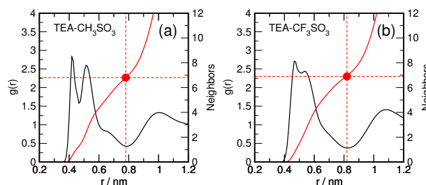
Fig. 4 Anion-cation center of mass pair distribution functions g(r) obtained for a) pure TEAMS and b) pure TEATF at T = 300 K. The position of the first minimum is used as a cut-off distance for the nearest neighbor computation (TEA-MS: 0.78 nm, TEA-TF: 0.81 nm).
