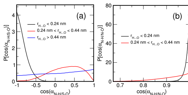
Fig. 10 Distribution of the cosine angles between two vectors for selected r_{H-O} -distance ranges. a) cosine angle between the N-H-vector in TEA and S-O vector in Methylsulfonate \cos(\alpha_{N-H/S-O}) b) cosine angle between N-H-vector in TEA and intermolecular N-O vectors \cos(\alpha_{N-H/N-O}) . Data is shown for TEA-Methylsulfonate pairs in a 50:50 TEAMS/TEATF-mixture at 300K. The pairs were preselected with respect to their intermolecular N-O distance using r_{N-O} < 0.8 nm.
