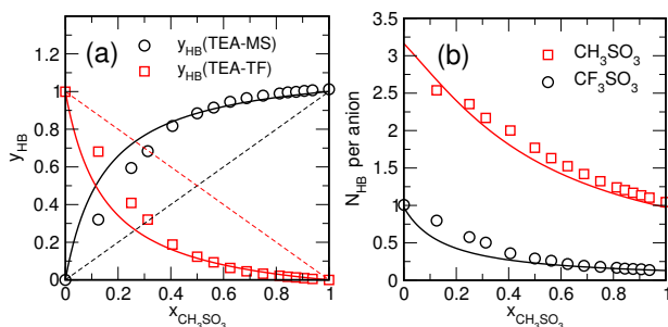
Fig. 16 a) Percentage of TEA-cations connected via a hydrogen bond to either a Triflate-ion or a Methylsulfonate-ion as a function of the mixture-composition. b) Average number of hydrogen bonds accepted by the Triflate- and Methylsulfonate-ions. Open Symbols: MD-data obtained at 400K. Solid lines: Model using equal statistical weights with w_{6,n} = 1 for n \leq 3 and w_{6,n} = 0 for n > 3 .
