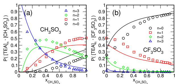
Fig. 15 Percentage of Methylsulfonate- (a) and Triflate-ions (b) hydrogen-bonded to zero, one, two, and three TEA-cations, as a function of the mixture-composition at 400K. Symbols: MD-simulation. Solid lines: Model using equal statistical weights with w_{6,n} = 1 for n \leq 3 and w_{6,n} = 0 for n > 3 .
