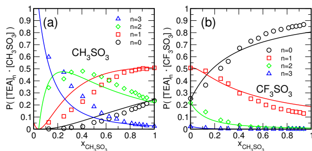
Fig. 17 Percentage of Methylsulfonate- (a) and Triflate-ions (b) hydrogen-bonded to zero, one, two, and three TEA-cations, as a function of the mixture-composition at 400K. Symbols: MD-simulation. Solid lines: Model using statistical weights adjusted to the distribution in the pure liquids with w_{6,0} = 0.75 , w_{6,1} = 1.3 , w_{6,2} = 1.12 , w_{6,3} = 0.5 , and w_{6,n} = 0 for n > 3 .
