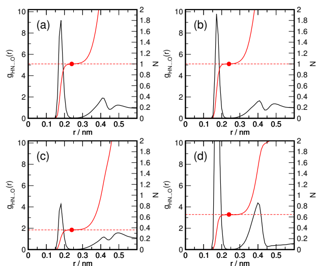
Fig. 8 H-O intermolecular site-site radial pair distribution functions g(r) obtained for pure TEATF and TEAMS ionic liquids and their 50:50 mixture at 300K. Also shown are the number of nearest neighbors as a function of distance N(r) . a) pure TEATF b) pure TEAMS c) H-O correlation between TEA and TF in the x_{MS} = 0.25 mixture d) H-O correlation between TEA and MS in the x_{MS} = 0.25 mixture.
