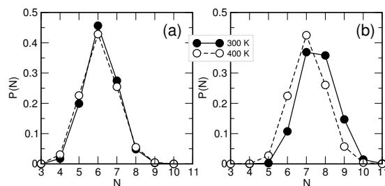
Fig. 7 Distribution of the number N of TEA-cations in the first solvation shell of the Triflate- and Methylsulfonate-anions in a 50:50 mixture of TEATF/TEAMS obtained for T = 300 K and T = 400 K. a) Methylsulfonate-TEA b) Triflate-TEA
