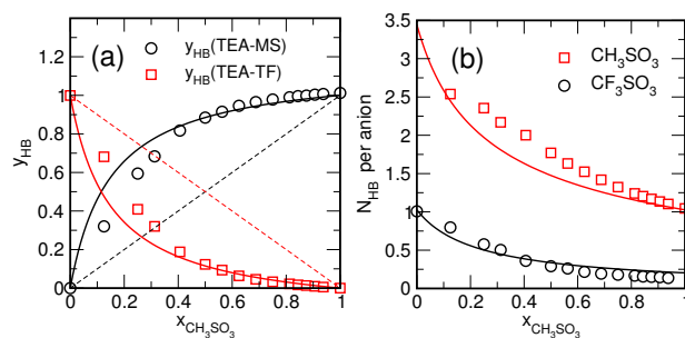
Fig. 18 a) Percentage of TEA-cations connected via a hydrogen bond to either a Triflate-ion or a Methylsulfonate-ion as a function of the mixture-composition. b) Average number of hydrogen bonds accepted by the Triflate- and Methylsulfonate-ions. Open Symbols: MD-data obtained at 400K. Solid lines: Model using statistical weights adjusted to the distribution in the pure liquids with w_{6,0} = 0.75 , w_{6,1} = 1.3 , w_{6,2} = 1.12 , w_{6,3} = 0.5 , and w_{6,n} = 0 for n > 3 .
