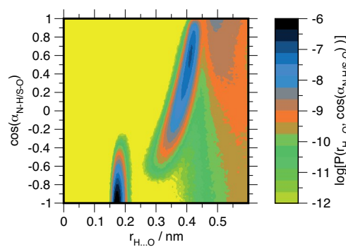
Fig. 9 Logarithmic representation of the probability-density of finding an intermolecular H-O distance r_{H-O} and the cosine angle between the respective N-H and S-O vectors \cos(\alpha_{N-H/S-O}) obtained for the TEA-Methylsulfonate pairs in a 50:50 TEAMS/TEATF-mixture at 300K. The pairs were preselected with respect to their intermolecular N-O distance using r_{N-O} < 0.8 nm.
