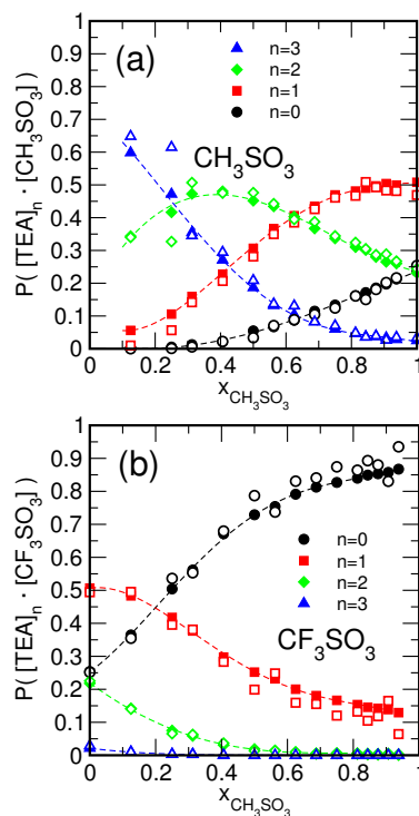
Fig. 13 Percentage of Triflate- and Methylsulfonate-ions hydrogen-bonded to zero, one, two, and three TEA-cations as a function of the mixture-composition. Open symbols: 300 K Closed symbols: 400 K a) Methylsulfonate b) Triflate.
