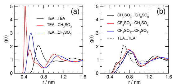
Fig. 3 Complete set of ion-ion center of mass pair distribution functions g(r) obtained for the 50:50 mixture of TEATF/TEAMS at T = 300 K.
