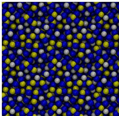
Fig. 2 Snapshot of a 50:50 mixture of TEATF/TEAMS at T = 300 K. The spheres represent the centers of gravity of the ions. The TEA-positions are indicated by blue spheres. The Triflate- and Methylsulfonate-positions are color-coded in white and yellow, respectively.
