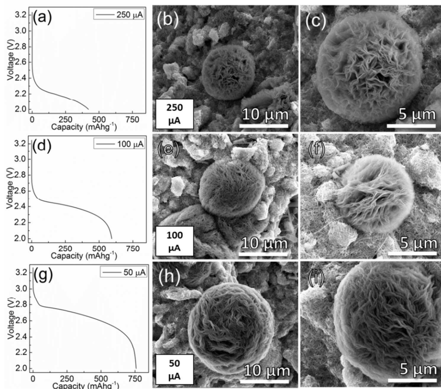
Fig.3: Discharge curves and SEM images of discharge products noted at different applied currents (250 \mu\text{A} (a,b,c), 100 \mu\text{A} (d,e,f) and 50 \mu\text{A} (g,h,i)) for single discharges of pure \text{MnO}_2 cathodes.
