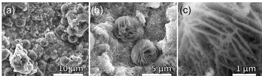
Fig.2: SEM images of a pure MnO 2 cathode discharged at a current rate of 100 mA g -1 . There are a number of large agglomerates covering the underlying MnO 2 . b) An example of two large plate agglomerates with the interlinked MnO 2 clearly visible in the background. c) High magnification image of single agglomerate.
