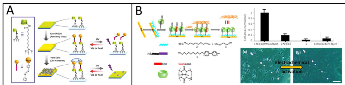
Figure 12. Supramolecular host-guest assemblies of a (A) photo-responsive \alpha -CD-host and azobenzene-RGD-guest (Reproduced with permission from ref. 123 provided by the American Chemical Society, 2014) and (B) electrochemically responsive CB[8]-host with two guests i.e. surface bound viologen and RGD-peptide functionalized tryptophan (Reproduced with permission from ref. 125 provided by John Wiley and Sons, 2014).
