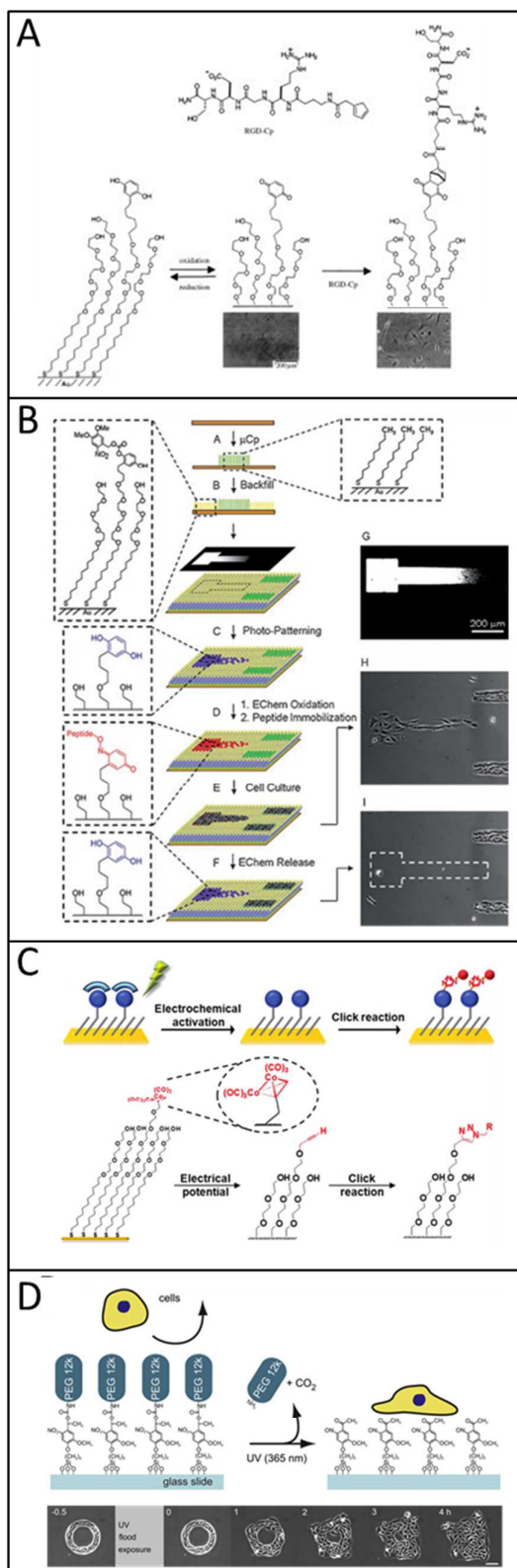
Figure 11. (A) HQ immobilized to gold substrates oxidizes to BQ and undergoes Diels-Alder reaction with RGD-cyclopentadiene (Cp). Attachment of RGD changes the substrate from cell-repellent to cell
