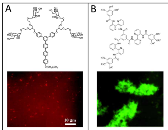
Figure 7. (A) A triblock rigid aromatic-flexible dendritic block molecules consisting of a hydrophobic alkyl chain ( n = 21 ), a rigid aromatic segment and flexible carbohydrate conjugate dendrons. The carbohydrate-coated nanostructures can immobilize E. Coli cells. The degrees of immobilization were significantly dependent on the shape of nanostructure (Reproduced with permission from ref. 63 provided by the American Chemical Society, 2014). (B) Discotic compounds functionalized with mannose ligands ( R_2 ) and inert glycol side chains ( R_1 ) form columnar architectures. Binding of these systems to bacteria result in their clustering, which was visualized using fluorescence microscopy (Reproduced with permission from ref. 64 provided by John Wiley and Sons, 2014).
