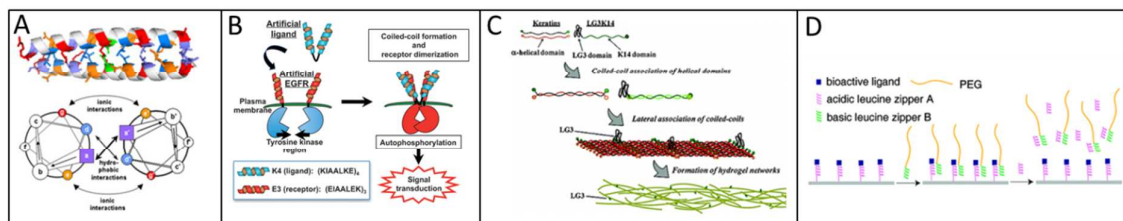
Figure 2. (A) Helical-wheel representation of a parallel dimer with a heptad repeat of amino acids present in assemblies of coiled-coil peptide motifs. The heptad repeat positions are labeled from a to g and the \alpha -helices propagate into the page. The a , d surface is predominantly hydrophobic, and residues at positions e and g are often charged (Reproduced with permission from ref. 29b provided by Springer, 2014). (B) Scheme of artificial activation of transmembrane receptors by a helical peptide through coiled-coil formation (Reproduced with permission from ref. 32 provided by John Wiley and Sons, 2014). (C) Schematic diagram showing the self-assembly of keratins in the presence of extracellular matrix protein domains (Reproduced with permission from ref. 36 provided by the American Chemical Society, 2014). (D) Illustration of the molecular design of bioactive surfaces capable of dynamically and reversibly regulating immobilized ligands using leucine zipper assembly (Reproduced with permission from ref. 37 provided by the American Chemical Society, 2014).
