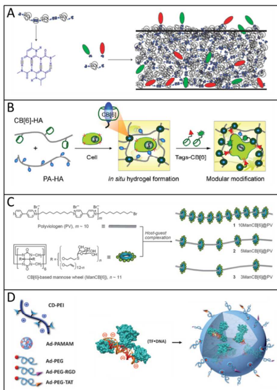
Figure 1. Schematic representations of (A) the self-complementary hydrogen-bonding Upy moiety in a supramolecular polymer that allows for the incorporation of different Upy-functionalized bioactive ligands (green and red moieties) by simply mixing the components (Reproduced with permission from ref. 13 provided by the Nature Publishing Group, 2014) and (B) the host-guest complexations between host CB[6]-conjugated biopolymers with guest polyamine-conjugated biopolymers to form a supramolecular hydrogel that allows simply mixing in of various bio-ligand tagged-CB[6] (Reproduced with permission from ref. 17 provided by the American Chemical Society, 2014) (C) Glyco-pseudopolyrotaxanes composed of various densities of CB[6]-based mannose wheels threaded on polyviologen showed the highest inhibitory potency for E. Coli ORN178-induced hemagglutination relative to monomeric mannoside studies in the case of the lowest density of wheels per chain (Reproduced with permission from ref. 23 provided by John Wiley and Sons, 2014). (D) Schematic representation of the host-guest self-assembly approach for the preparation of supramolecular nanoparticles by simply mixing host CD-functionalized polymers to complex guest Ad-functionalized
