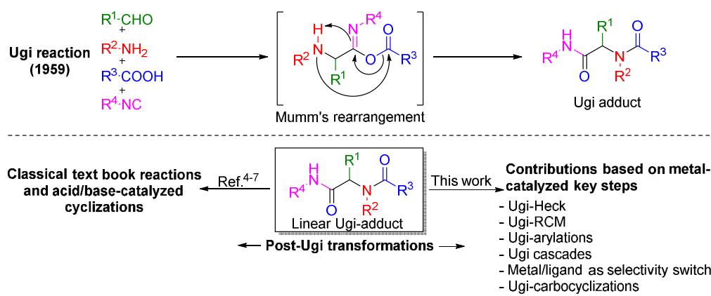
Figure 1 Ugi-4CR and post-transformations for the generation of diverse heterocycles.
