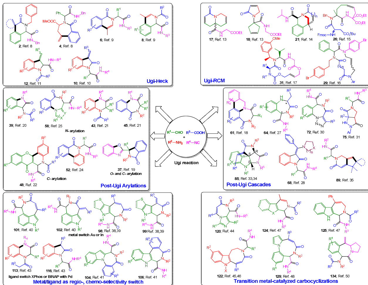
Figure 2 Overview of transition metal-catalyzed post-Ugi transformations.
