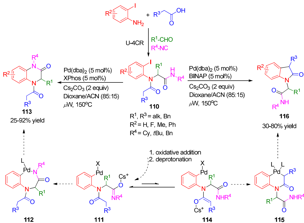
Scheme 31 Regioselective synthesis of 5,6-dihydroindolo[1,2- a ]quinoxalines and 6,7-dihydroindolo[2,3- c ]quinolones.
