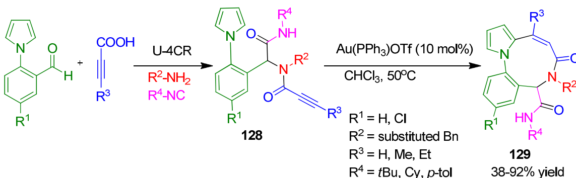
Scheme 35 Synthesis of diversely substituted diazoninones via Au-catalyzed carbocyclization.
